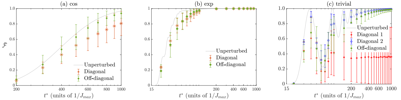
FIG. 6. For each protocol, (a) cosine, (b) exponential and (c) trivial, we show the impact of diagonal and off-diagonal disorder of strength d_s = 0.2 (units of J_{\max} ). Each point corresponds to the mean value of the transfer probability \bar{\mathcal{F}} averaged over 10 000 disorder realizations given as a function of the transfer time, while the error bars correspond to the standard deviation of the sample. In order to compare we have also included the unperturbed curve. The transfer time axis is displayed in logarithmic scale. We also note that the limits of the t^* axis for the cosine differ from the other two.
