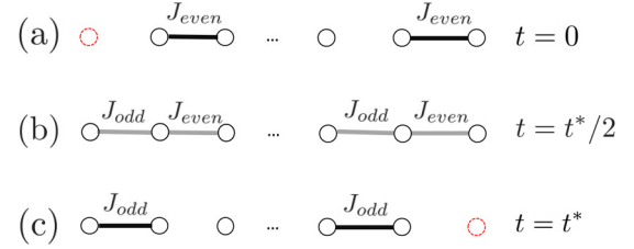
FIG. 1. A schematic of different time instants during the dynamical evolution of the topological chain. (a) Initially, J_{\text{odd}} = 0 , J_{\text{even}} = J_{\text{max}} , the zero mode is localized on the first site, and the energy gap takes its maximum value. (b) For t = t^*/2 , we have J_{\text{even}} = J_{\text{odd}} < J_{\text{max}} and the energy gap acquires its minimum value. Before and after t^*/2 , we have J_{\text{odd}} < J_{\text{even}} < J_{\text{max}} and J_{\text{even}} < J_{\text{odd}} < J_{\text{max}} , respectively. (c) Finally, J_{\text{odd}} = J_{\text{max}} , J_{\text{even}} = 0 , the zero mode is localized on the last site, and the energy gap once again takes its maximum value.
