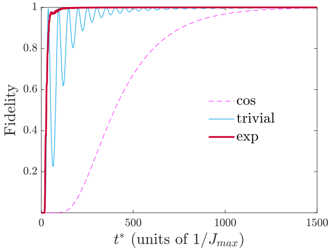
FIG. 4. Fidelity as a function of the transfer time for all protocols.
