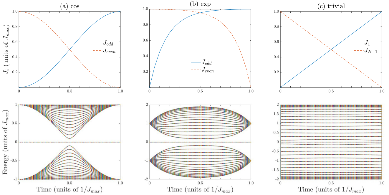
FIG. 3. For each protocol, (a) cosine, (b) exponential, and (c) trivial, in the top panel we plot the driving function as a function of time. While in the bottom panel, we depict the corresponding instantaneous energy spectrum as a function of time. In all plots, we have taken the transfer time to be t^* = 1 and the chain consists of N = 31 sites.
