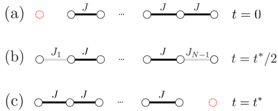
FIG. 2. A schematic of different time instants during the dynamical evolution of the topologically trivial chain. (a) Initially, J_1 = 0 and J_i = J_{\max} , where i = 2, \dots, N-1 , the zero mode is localized on the first site, and the energy gap takes its maximum value. (b) For t = t^*/2 , we have J_1 = J_{N-1} < J_{\max} , while J_i = J_{\max} for i = 2, 3, \dots, J_{N-2} . Before and after t^*/2 , we have J_1 < J_{N-1} < J_{\max} and J_{N-1} < J_1 < J_{\max} , respectively. (c) Finally, J_1 = 0 and J_i = J_{\max} for i = 2, \dots, N-1 , while the zero mode is localized at the last site of the chain.
