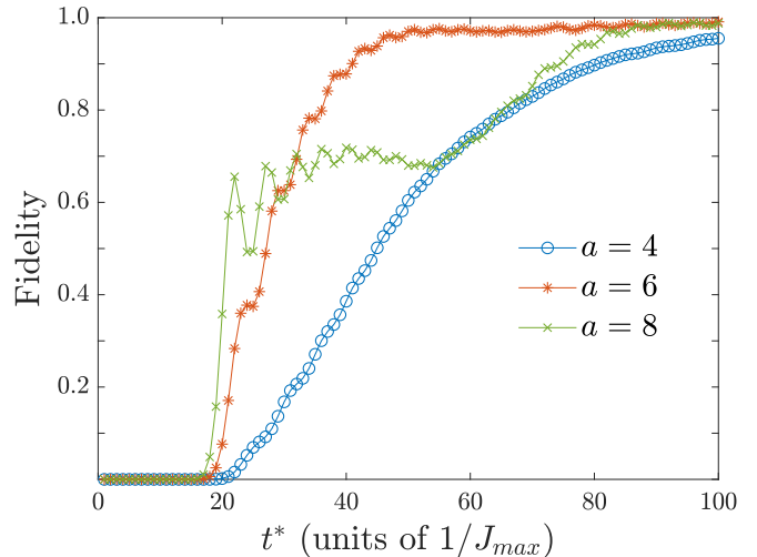
FIG. 5. Fidelity as a function of the transfer time for the exponential driving and for different values of the \alpha parameter.
