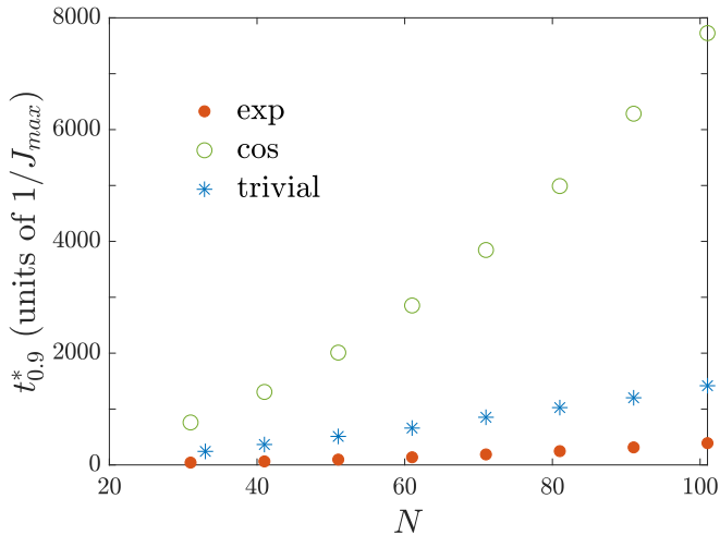
FIG. 7. For each protocol, we plot the transfer time t_{0.9}^* it takes to reach \mathcal{F} = 0.9 as a function of the system's size N .
