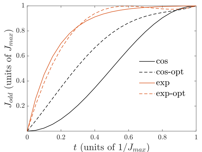
FIG. 8. For the protocol employing the SSH chain, we plot the coupling strength J_{\text{odd}} as a function of time t for the cosine (black line) and the exponential (red line) driving, together with the corresponding optimized driving functions (black dashed line for the cosine and red dashed line for the exponential) obtained by the optimal control method CRAB. Note that the driving function imposed on J_{\text{even}} is obtained by mirror inverting this picture, where the axis of symmetry has the equation t = 0.5 .
