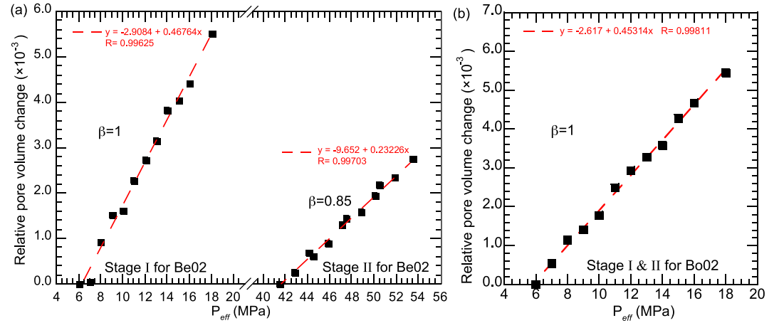
Figure 7. Relative pore volume change as a function of effective stress for (a) Berea (Be02) and (b) Boise (Bo02) sandstones. The effective stress was calculated using values of the effective stress coefficients for pore volume change \beta indicated on the graphs. The measurements are shown as black squares. The red lines correspond to linear fits based on the equations shown on the graphs.
