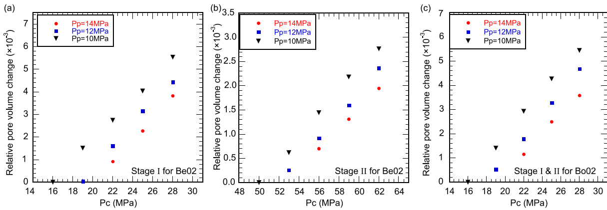
Figure 5. Relative pore volume change as a function of confining pressure for three different pore pressures of Berea and Boise sandstones: (a) stage I for BeO2, (b) stage II for BeO2, (c) stages I and II for BoO2.
