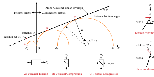
Figure 1 The Mohr–Coulomb criterion for the elements
