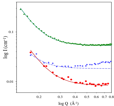
FIG. 12: Log-log plot of the scattered intensity at low Q for the three different deuterations of the glycerol-water solution with c_g = 0.178 at 160 K at the end of the annealing when water has crystallized: same data and color code as in Fig. 1 of the main text. The lines are the best fits to Porod’s law, I(Q) = aQ^{-4} + b . The fit to the C_3H_5(OD)_3 + D_2O data (dashed blue line and symbols) is only indicative as over the range of probed wavevectors the Porod regime does not emerge distinctly enough.
