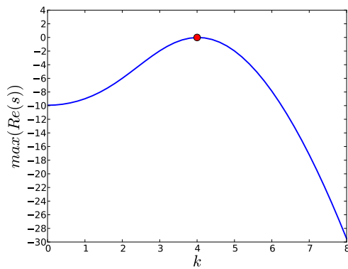
(a) Growth rate ( \sim \max(\text{Re}(s)) ) depending on k . The red dot represents the k_c = 4.0 where \max(\text{Re}(s)) = 0 .
