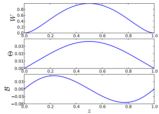
(b) Eigenvectors for k = k_c = 4.0 .
