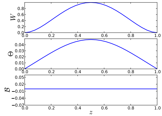
(b) Eigenvectors for k = k_c = 3.14 .
