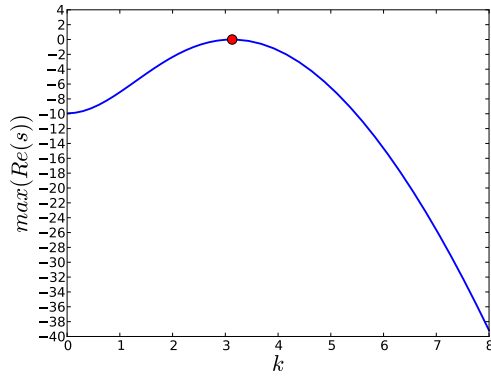
(a) Growth rate ( \sim \max(\text{Re}(s)) ) depending on k . The red dot represents the k_c = 3.14 where \max(\text{Re}(s)) = 0 .
