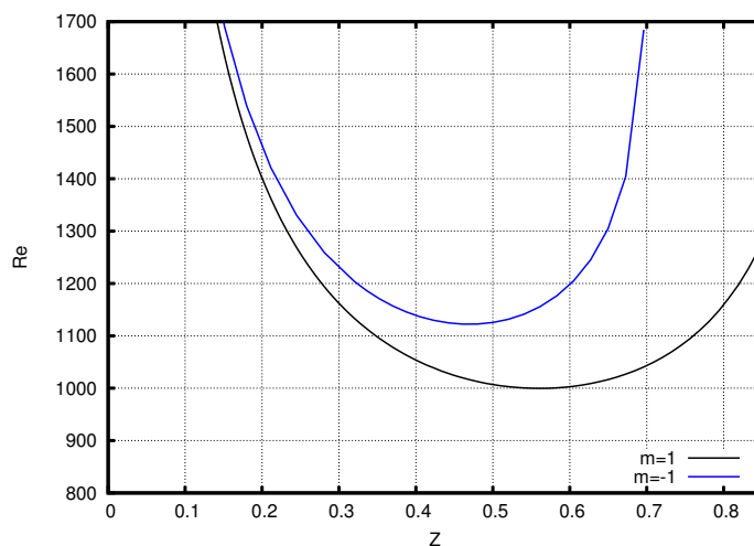
Figure 6: Neutral curves at S = 0.0005 for m = 1 and m = -1 .
