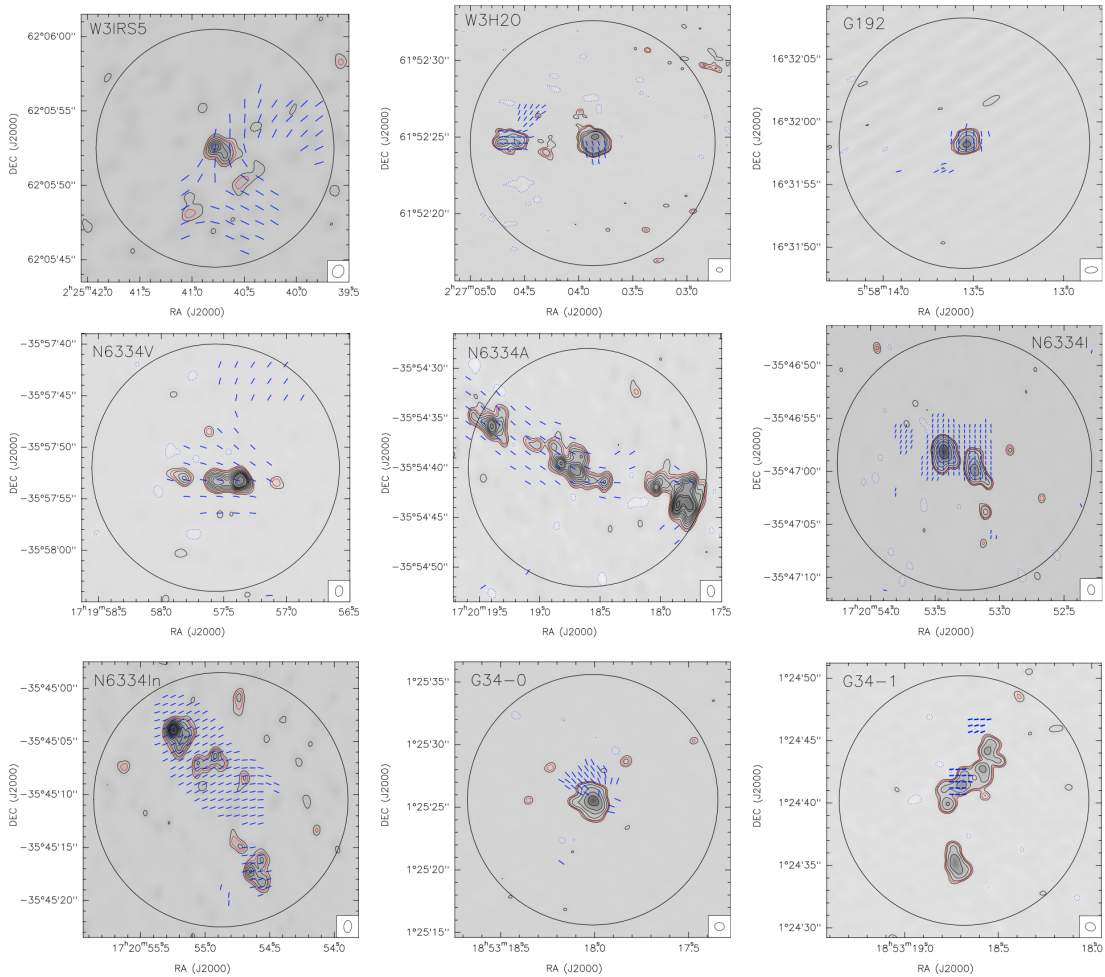
Figure 2a. 0.87 or 1.3 mm continuum high angular resolution maps with the magnetic field segments overplotted in blue. Contours for all regions are -4, 4, 8, 12, 16, 20, 24, 28, 36, 40, 50, 60, 70, 80, 100 and 120 times the rms noise, listed in Table 1, except for G192, N6334I, G34-0, and G34-1, for which contours are -4, 4, 8, 16, 32, 64, and 128 times the rms noise. For W3H2O contours are -4, 4, 8, 16, 24, 32, 64, 120 times the rms noise. Synthesized beams are plotted in the bottom-right corner of each panel, and the black circle corresponds to the common field of view of 0.15 pc diameter.
