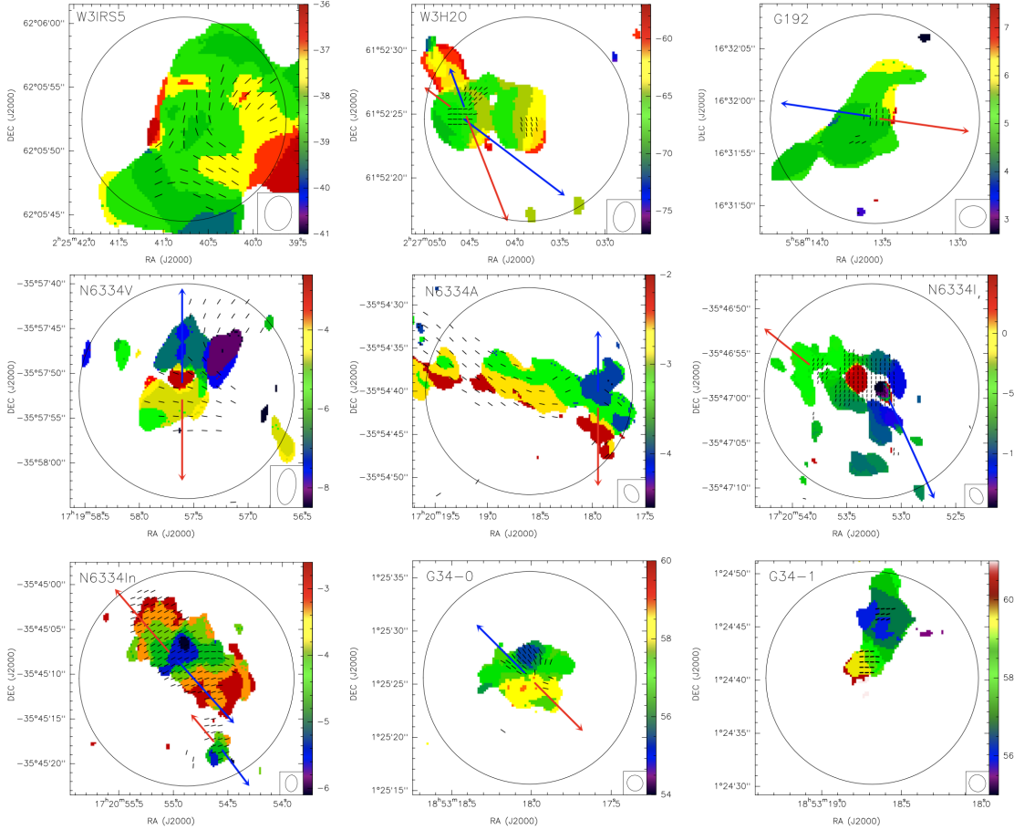
Figure 14a. First-order moments for \text{H}^{13}\text{CO}^+ (4–3) data with the magnetic field segments (black) overplotted. Red and blue arrows indicate the approximate orientations of the redshifted and blueshifted outflow emission according to Zapata et al. (2011), and Zhang et al. (2014). The synthesized beam is shown in the bottom-right corner. The circle corresponds to the field of view of 0.15 pc of diameter used in this work to assess the magnetic field strength. Wedge units are \text{km s}^{-1} .
