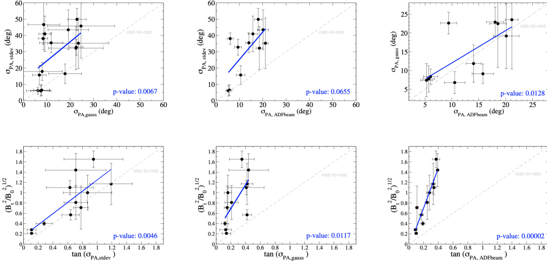
Figure 9. Comparison of the four different approaches used here to estimate \delta B/B_0 (Sections 4.3.1, 4.3.2, 4.4.1, and 4.4.2), with the results of linear regression fits (blue line) and the p-values (probability that the null hypothesis is true) listed in each panel. The grey dashed line indicates the one-to-one relation.
