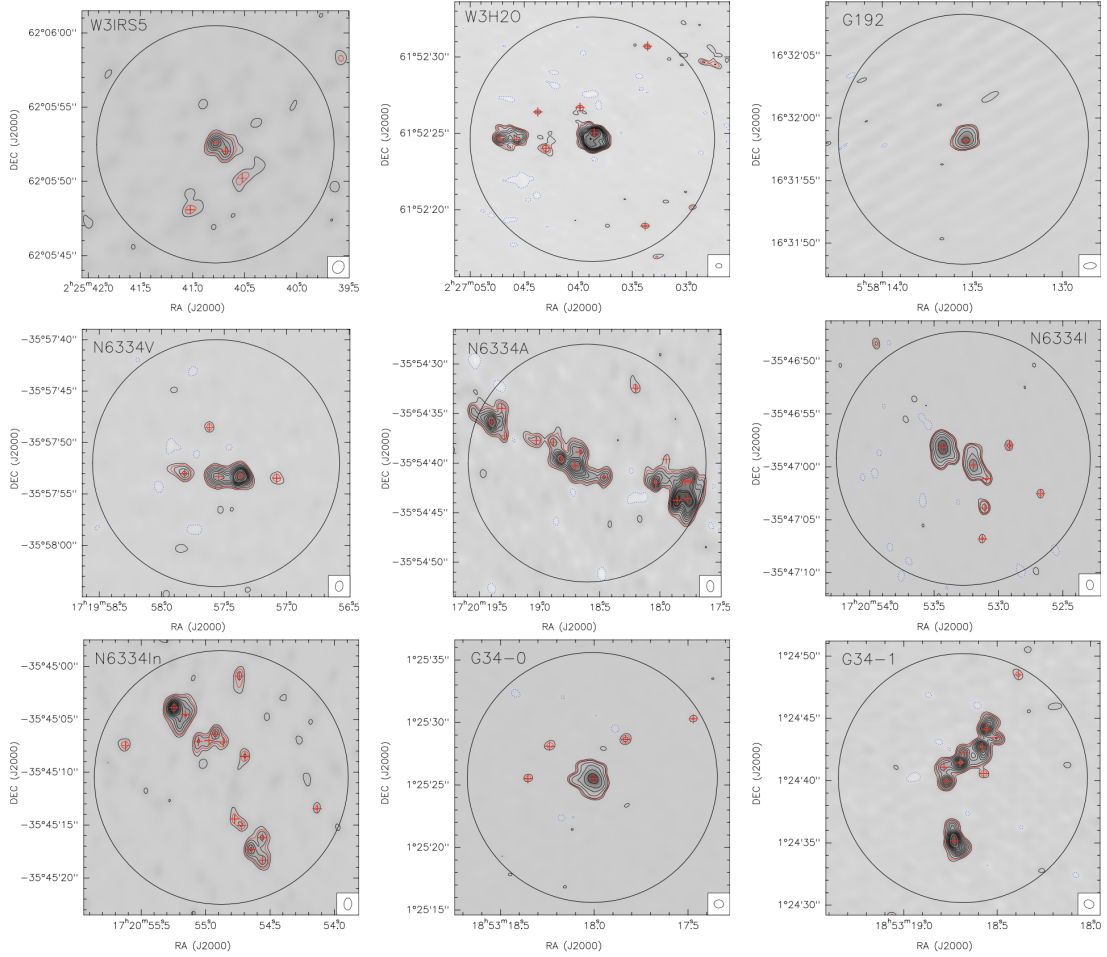
Figure 1a. 0.87 or 1.3 mm continuum high angular resolution maps. Contours for all regions are -4, 4, 8, 12, 16, 20, 24, 28, 36, 40, 50, 60, 70, 80, 100 and 120 times the rms noise, listed in Table 1, except for G192, N6334I, and G34-0, for which contours are -4, 4, 8, 16, 32, 64, and 128 times the rms noise. Synthesized beams are plotted in the bottom-right corner of each panel, and the black circle corresponds to a field of view of 0.15 pc diameter (the field of view common to all the regions, given their primary beams). In all panels the red contour corresponds to the identification level of 6\sigma , and the plus signs correspond to the identified fragments.
