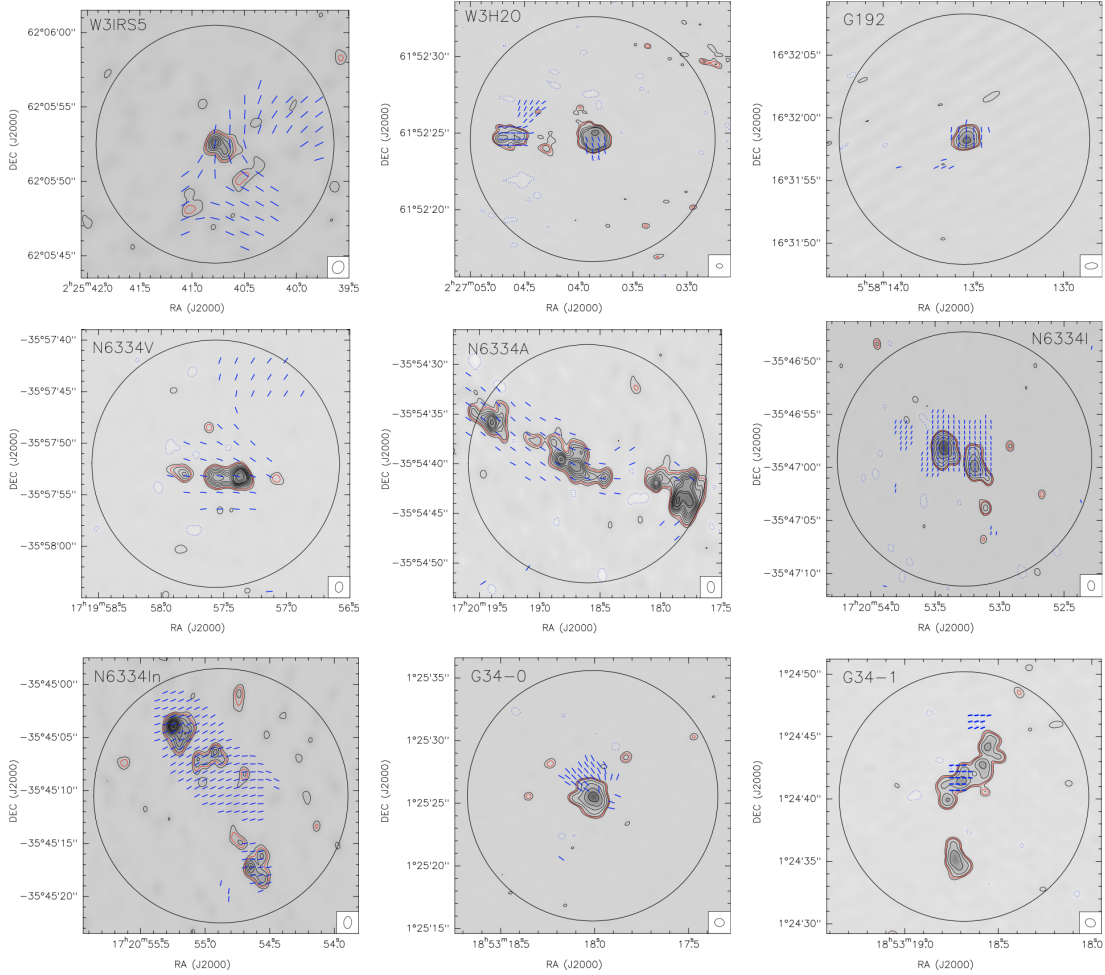
Figure 2a. 0.87 or 1.3 mm continuum high angular resolution maps with the magnetic field segments overplotted in blue. Contours for all regions are -4, 4, 8, 12, 16, 20, 24, 28, 36, 40, 50, 60, 70, 80, 100 and 120 times the rms noise, listed in Table 1, except for G192, N6334I, G34-0, and G34-1, for which contours are -4, 4, 8, 16, 32, 64, and 128 times the rms noise. For W3H2O contours are -4, 4, 8, 16, 24, 32, 64, 120 times the rms noise. Synthesized beams are plotted in the bottom-right corner of each panel, and the black circle corresponds to the common field of view of 0.15 pc diameter.
