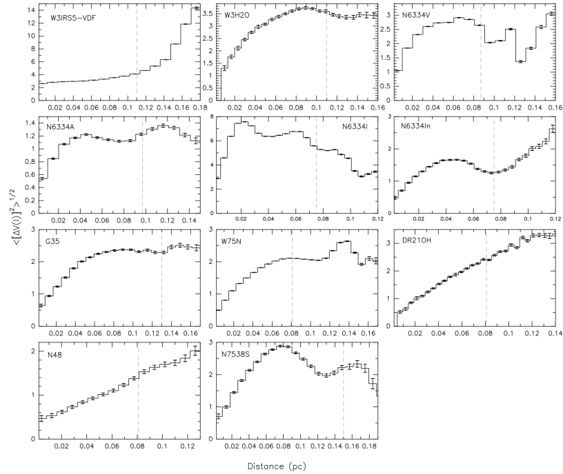
Figure 5. Velocity Dispersion Functions in \text{km s}^{-1} (i. e., \langle [\Delta V(\ell)]^2 \rangle^{1/2} , as defined in equation 2), for the regions for which the ADF (Section 4.4) was also calculated, measured using the \text{H}^{13}\text{CO}^+ (4-3) first-order moment maps of Figs. 14a and 14b. The dashed grey vertical line indicates the largest angular scale that the SMA is able to recover for the \text{H}^{13}\text{CO}^+ (4-3) emission.
