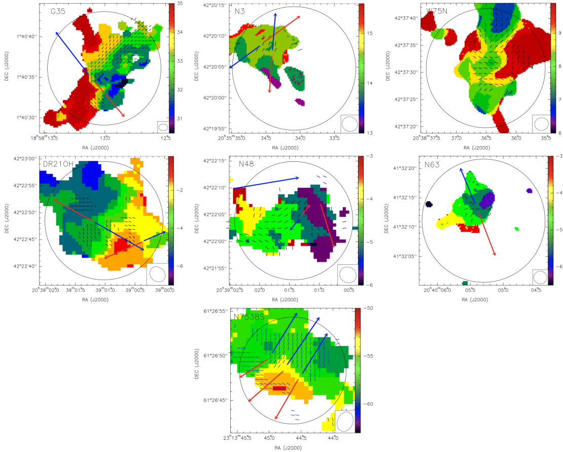
Figure 14b. First-order moments for \text{H}^{13}\text{CO}^+ (4–3) data with the magnetic field segments (black) overplotted. Red and blue arrows indicate the approximate orientations of the redshifted and blueshifted outflow emission according to Naranjo-Romero et al. (2012), Duarte-Cabral et al. (2013, 2014), Girart et al. (2013), and Zhang et al. (2014). The synthesized beam is shown in the bottom-right corner. The circle corresponds to the field of view of 0.15 pc of diameter used in this work to assess the magnetic field strength. Wedge units are \text{km s}^{-1} .
