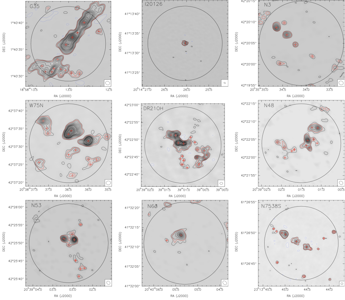
Figure 1b. 0.87 or 1.3 mm continuum high angular resolution maps. Contours for all regions are -4, 4, 8, 12, 16, 20, 24, 28, 36, 40, 50, 60, 70, 80, 100 and 120 times the rms noise, listed in Table 1, except for I20126, N63, and N7538S for which contours are -4, 4, 8, 16, 32, (48), 64, and 128 times the rms noise, and for G35, for which contours are -4, 4, 8, 12, 20, 28, 36, 44, 52, 60, 80, 100, 120, 150 and 200 times the rms noise. Synthesized beams are plotted in the bottom-right corner of each panel, and the black circle corresponds to a field of view of 0.15 pc diameter (the field of view common to all the regions, given their primary beams). In all panels the red contour corresponds to the identification level of 6\sigma , and the plus signs correspond to the identified fragments.
