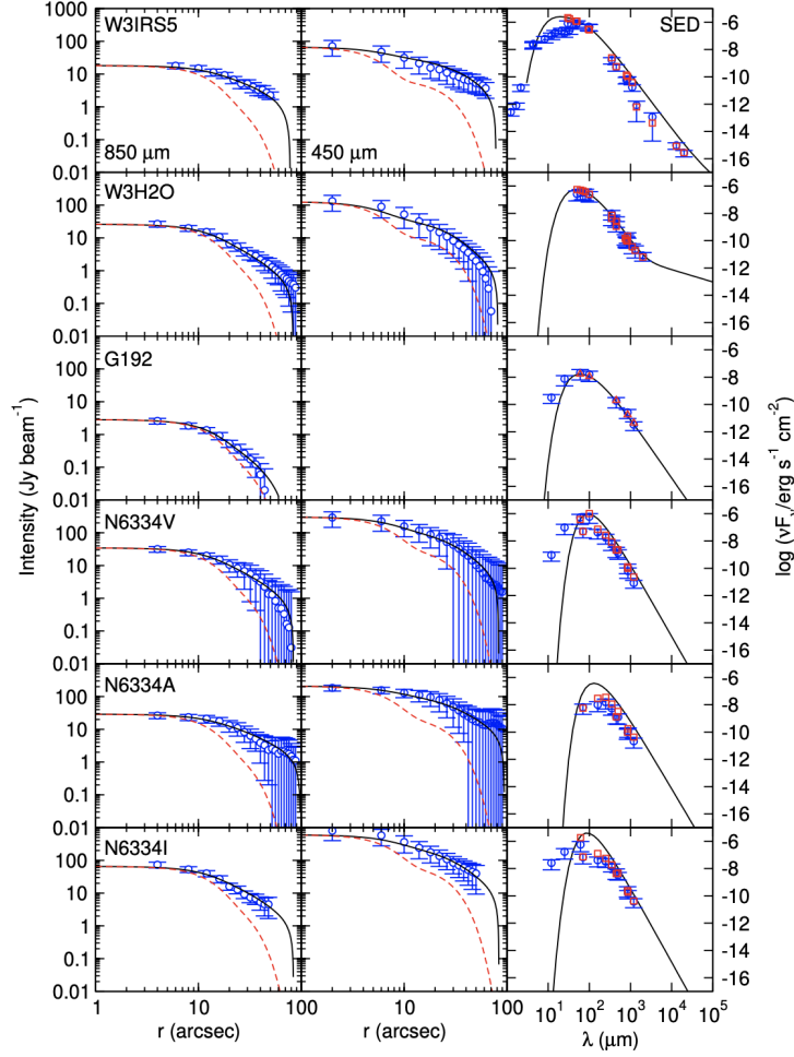
Figure 3a. Best fits for six regions of the sample (see Table 3 for the exact fitted parameters). Each row corresponds to one core, the left (middle) panel shows the radial intensity profile at 850 (450) \mu\text{m} , with the empty blue circles corresponding to the data, the black solid line corresponding to the model, and the dashed red line showing the beam profile; panels on the right show the SED, with blue empty circles indicating the observed fluxes, the black solid line showing the model for a fixed aperture, and the red squares corresponding to the model for the same aperture where each flux was measured.
