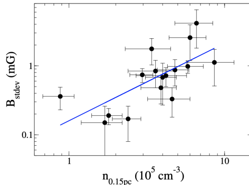
Figure 15. Magnetic field strength calculated with the ‘standard deviation’ approach, B_{\text{stddev}} , vs density averaged within 0.15 pc. The blue line corresponds to a linear fit in logarithmic scales with a slope of 1.1 \pm 0.3 and a correlation coefficient of 0.69.
