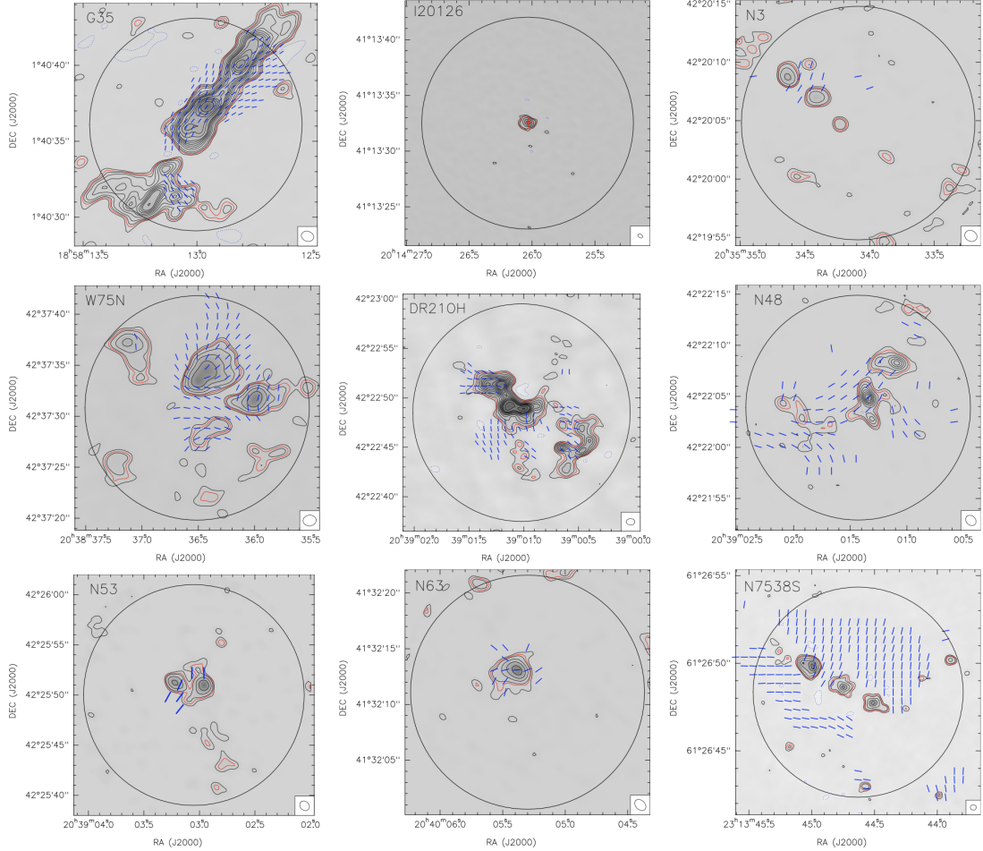
Figure 2b. 0.87 or 1.3 mm continuum high angular resolution maps with the magnetic field segments overplotted in blue. Contours for all regions are -4, 4, 8, 12, 16, 20, 24, 28, 36, 40, 50, 60, 70, 80, 100 and 120 times the rms noise, listed in Table 1, except for I20126, W75N, N53, N63 and N7538S for which contours are -4, 4, 8, 16, 32, 64, and 128 times the rms noise, and for G35, for which contours are -4, 4, 8, 12, 20, 28, 36, 44, 52, 60, 80, 100, 120, 150 and 200 times the rms noise. Synthesized beams are plotted in the bottom-right corner of each panel, and the black circle corresponds to the common field of view of 0.15 pc diameter.
