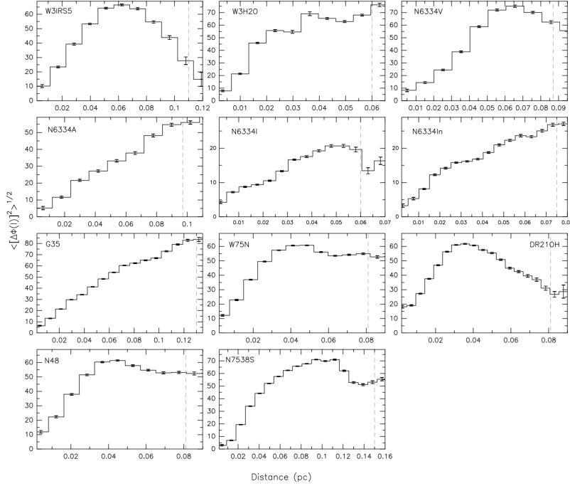
Figure 7. ADF (i. e., \langle [\Delta\Phi(\ell)]^2 \rangle^{1/2} , as defined in equation 7) for each region with enough polarization detections. The dashed grey vertical line indicates the largest angular scale that the SMA is able to recover for the polarized emission.
