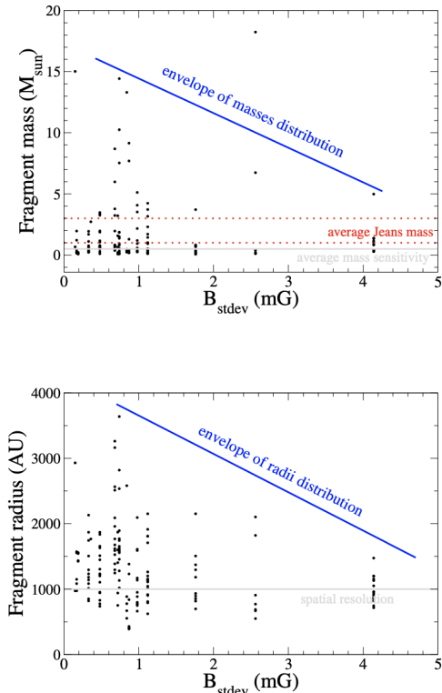
Figure 12. Top: Masses of the fragments identified within each massive dense core vs B_{\text{stdev}} . The horizontal red dotted lines indicate the range of average M_{\text{Jeans}} found for our sample assuming T = 20 K and T = T_{0.15\text{pc}} (Table 2). The horizontal grey line indicates the typical mass sensitivity of our observations (Table 1). Bottom: Radii (at the 3\sigma contour) of the fragments identified within each massive dense core vs B_{\text{stdev}} . The horizontal grey line indicates the typical spatial resolution of our observations (Table 1). Oblique lines are drawn to guide the eye.
