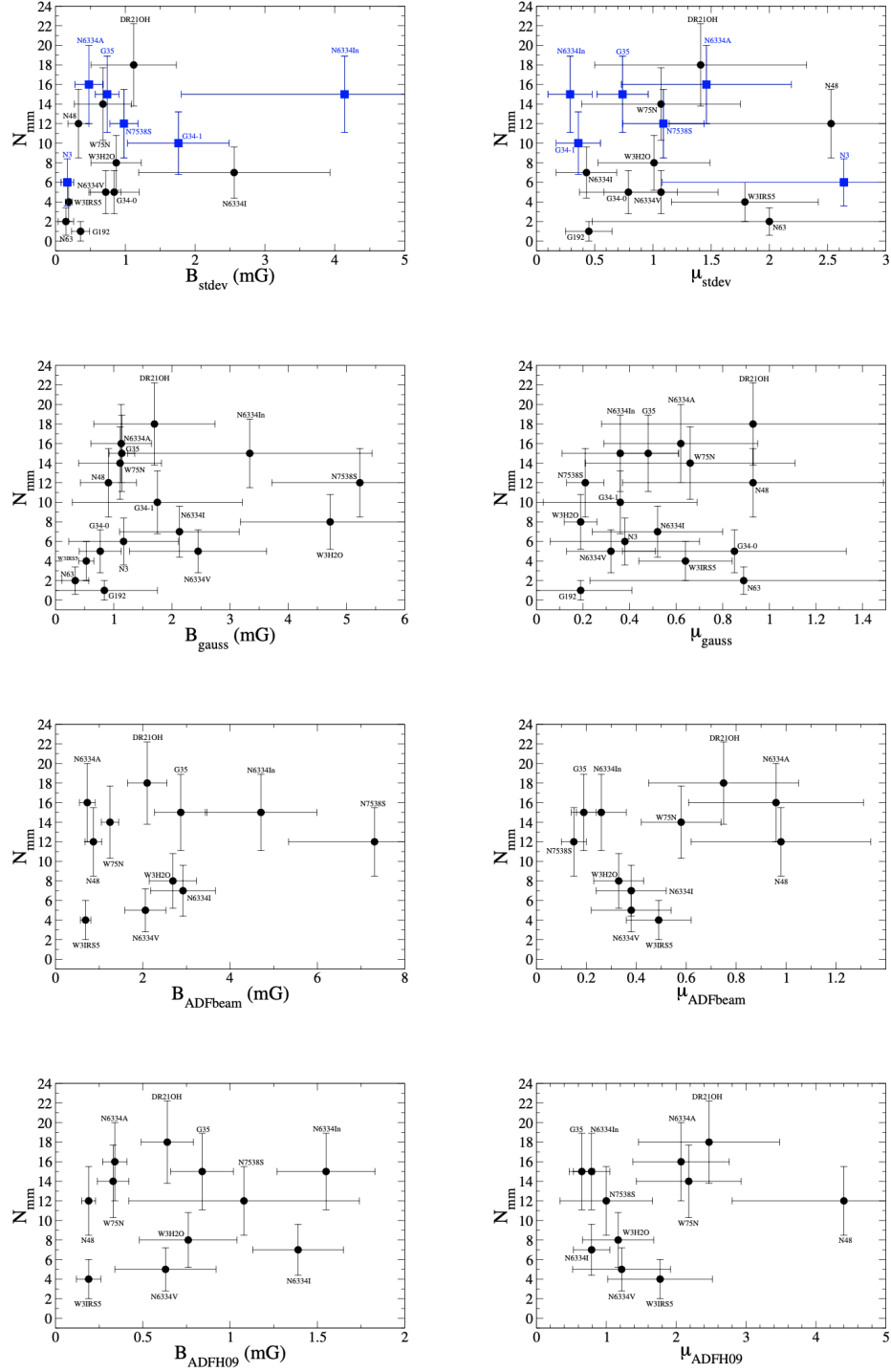
Figure 10. The four panels on the left show the plots of N_{\text{mm}} vs the magnetic field strength for the different approaches used in this work: ‘standard deviation’ ( B_{\text{stddev}} ), ‘multiple gaussian’ ( B_{\text{gauss}} ), ‘ADF beam’ ( B_{\text{ADFbeam}} ), and ‘ADF H09’ ( B_{\text{ADFH09}} ). The four panels on the right show the plots of N_{\text{mm}} vs the ratio of mass-to-flux to critical mass-to-flux, \mu , for the same four approaches. In the top panels, the blue squares correspond to the cores classified as presenting ‘aligned fragmentation’ in Table 2.
