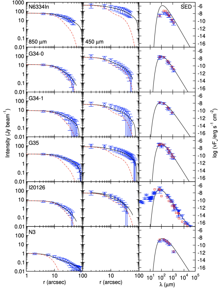
Figure 3b. Same as Fig. 3a.
