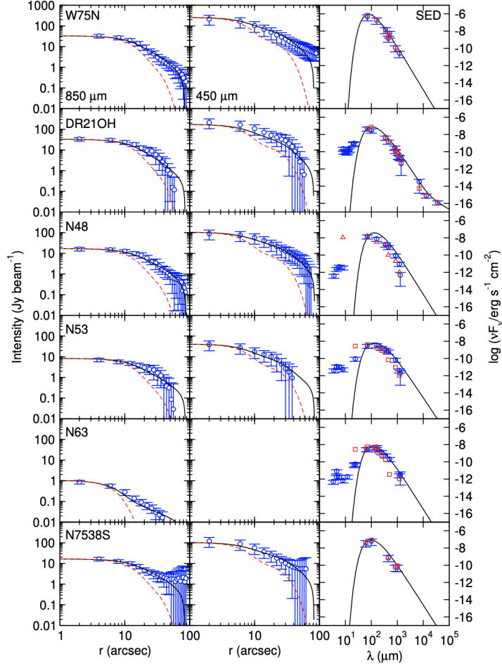
Figure 3c. Same as Fig. 3a.
