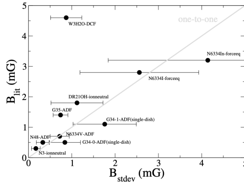
Figure 17. Comparison of the magnetic field determined in the literature and the magnetic field determined in this work using the ‘standard deviation’ approach, B_{\text{stdev}} . The light grey line corresponds to the one-to-one relation to guide the eye. Next to the name of each source, there is a short-name for the method used to determine the magnetic field strength. See Table 5 for further details.
