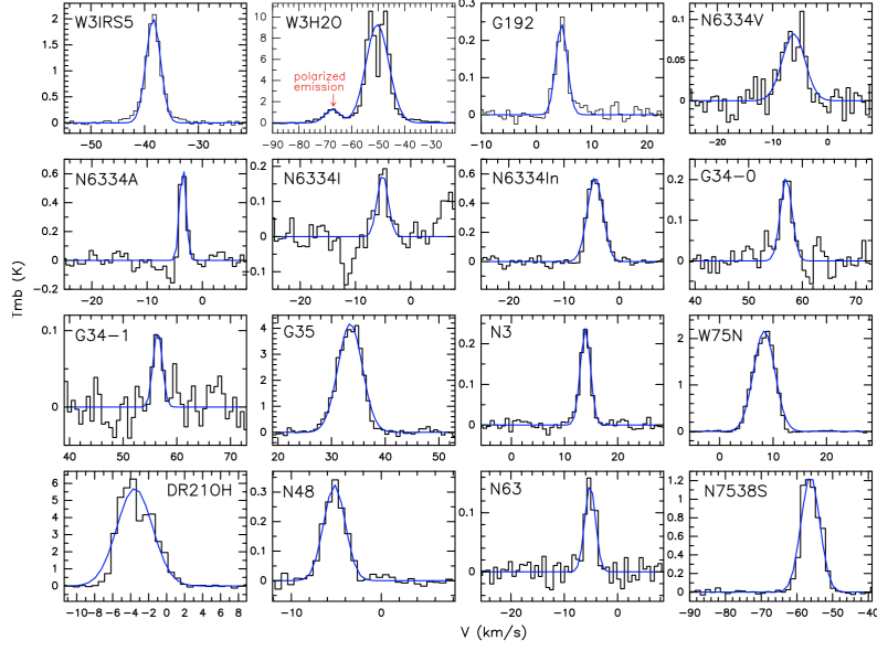
Figure 4. \text{H}^{13}\text{CO}^+ (4-3) spectra (black) with the gaussian fits (blue curves) performed to estimate the velocity dispersion in each region. For the case of W3H2O, the velocity component associated with the polarized emission is marked with a red arrow.
