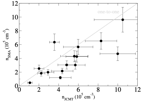
Figure 16. Plot of the SMA average density (within 0.15 pc of diameter) vs the average density inferred using the modeling of the single-dish data presented in Section 4.1. The light grey line indicates the one-to-one relation to guide the eye. To make the comparison, we converted the densities reported in Table 3, n_{0.15\text{pc}} , from density of \text{H}_2 particles to total density of particles. The uncertainties for the SMA average density have been adopted to be 20%, the typical uncertainty in the flux absolute scale.
