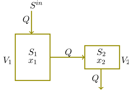
FIGURE 1. The serial configuration of two chemostats.
