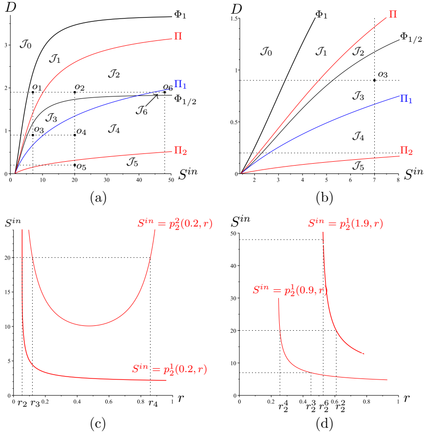
FIGURE 17. (a) and (b): The curves \Phi_1 , \Phi_{1/2} (in black), \Pi_1 (in blue), \Pi and \Pi_2 (in red) divide the operating plane in seven regions, \mathcal{J}_k , k = 0..6 and the operating points o_k \in \mathcal{J}_k , k = 1..6 . (c): The graphical depiction of Assumptions 6 and 7, for D = 0.2 , showing the values r_2 = r_2(S^{in}, D) , r_3 = r_3(S^{in}, D) and r_4 = r_4(S^{in}, D) , corresponding to o_5 . (d): The graphical depiction of Assumption 6, for D = 0.9 and D = 1.9 , showing the values r_2^k = r_2(S^{in}, D) , corresponding to o_k , k = 2, 3, 4, 6 , respectively. The operating points are o_1 = (8, 1.9) , o_2 = (20, 1.9) , o_3 = (8, 0.9) , o_4 = (20, 0.9) , o_5 = (20, 0.2) . and o_6 = (48, 1.9) .
