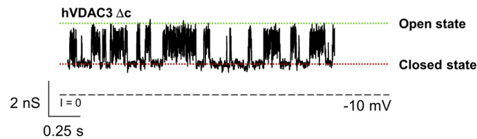
Figure S9. VDAC3- \Delta c recurrently forms low-conducting pores with flickering current. Representative single-channel current trace obtained with reconstituted VDAC3- \Delta c at -10 mV applied voltage. Dashed line indicates zero current level. Current records were digitally filtered at 500 Hz using a low-pass Bessel (8-pole) filter. Membranes were formed from DOPC/DOPE/2DOPG. Membrane-bathing solutions consisted of 1 M KCl buffered with 5 mM HEPES at pH 7.4.
