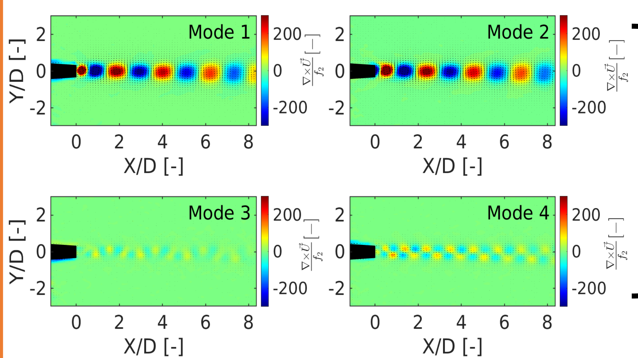
(x,y) cartography of vorticity at U_0 = 4.4 m/s, with shunt.
