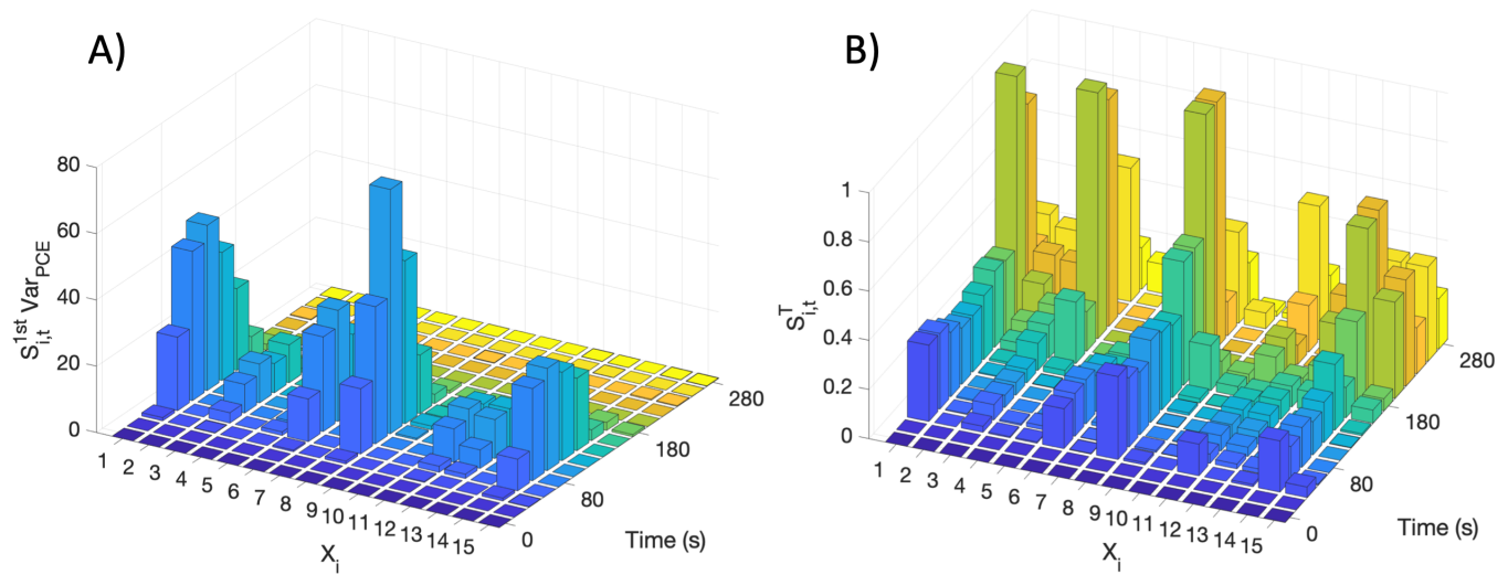
FIGURE 9 Sobol' indices evolution over time for the QoI closure percentage. A) First order indices multiplied by the output PCE variance. B) Total Sobol' indices.
