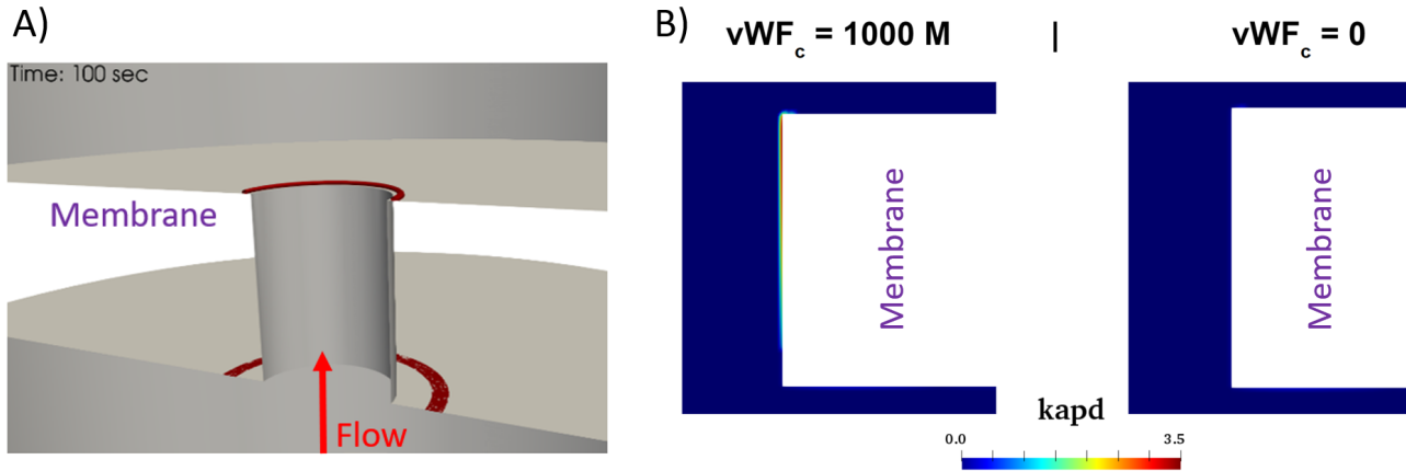
FIGURE 5 Thrombosis simulation with inlet condition vWF_c = 0 which corresponds to the original model of Wu et al. 33 . A) Lack of thrombus formation at 100 seconds with inlet boundary condition vWF_c = 0 . B) Platelet deposition rate k_{apd} with and without vWF_c .
