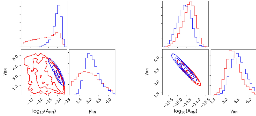
Figure 4. 2D distributions of achromatic red-noise amplitude and spectral index. Left plot: J1600–3053, the model RN\_DMv is in blue and RN\_DMv\_Sv is in red; Right plot: J1909–3744, with RN\_DMv in blue and RN\_DMv\_Sv (favourable) in red.
