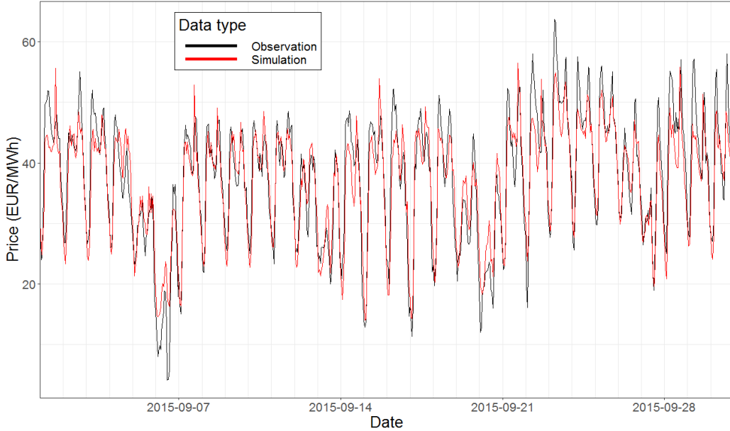
Figure 4: Time series of prices on the French day-ahead market over one month
