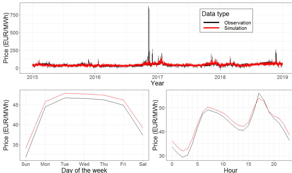
Figure 3: Time series of prices on the French day-ahead market over four years (top), average prices by day of the week (bottom-left) and average prices by hour of the day (bottom-right)
