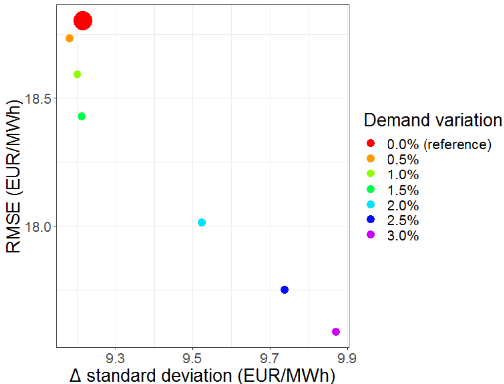
Figure 6: Out-of-sample performance for different augmented data sets (training set: 2015, testing set: 2016)
