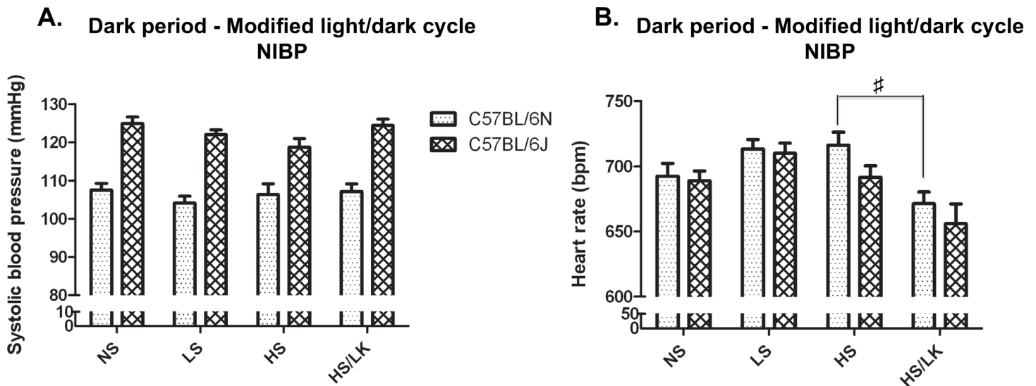
Fig 5. Comparison between C57BL/6N and C57BL/6J for their systolic blood pressure and heart rate responses to various salt challenges measured by NIBP. Measurements were made during the dark periods of a modified light/dark cycle. NS = normal salt diet (n = 20 and n = 20, for C57BL/6N and C57BL/6J respectively), LS = low salt diet (n = 20 and n = 20, for C57BL/6N and C57BL/6J respectively), HS = high Na + /normal K + diet (n = 9 and n = 10, for C57BL/6N and C57BL/6J respectively) and HS/LK = high Na + /low K + diet (n = 9 and n = 10, for C57BL/6N and C57BL/6J respectively). One-way ANOVA per light phase followed by Tukey Kramer's post-hoc test; #: p<0.05 HS/LK compared to HS.
