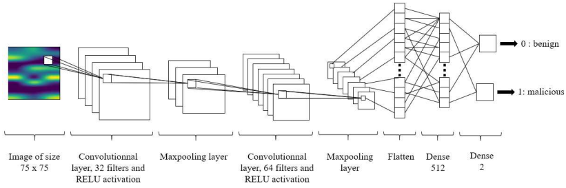
Fig. 6. VizNN architecture
