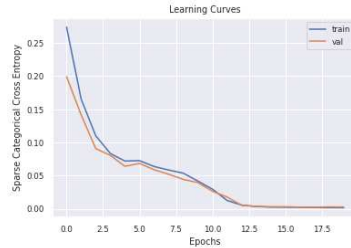
Fig. 10. The learning curves for VizNN Model
