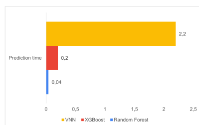
Fig. 13. Comparison of prediction time
