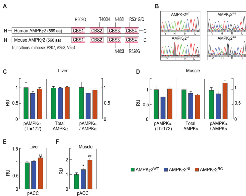
FIGURE 1. Characterization of AMPK \gamma 2 NI and AMPK \gamma 2 RG mice. A , schematic diagram of human and mouse AMPK \gamma 2 protein. Mouse AMPK \gamma 2 has three amino acid deletions, Pro-207, Ala-253, and Val-254, versus the human protein; thus, N485I and R528G correspond to N488I and R531G in human AMPK \gamma 2. B , modified sequence of AMPK \gamma 2 WT , AMPK \gamma 2 NI , and AMPK \gamma 2 RG mice. C and D , phosphorylated AMPK \alpha (Thr-172), total AMPK \alpha , and phospho-AMPK \alpha (Thr-172)/total AMPK \alpha ratio in liver and skeletal muscle of AMPK \gamma 2 WT , AMPK \gamma 2 NI , and AMPK \gamma 2 RG mice at 26 weeks of age ( n = 8 ). E and F , phosphorylated ACC in liver and skeletal muscle of AMPK \gamma 2 WT , AMPK \gamma 2 NI , and AMPK \gamma 2 RG mice at 26 weeks of age ( n = 8 ). RU, relative units. *, p \leq 0.05 ; **, p \leq 0.01 . Error bars, S.E.
