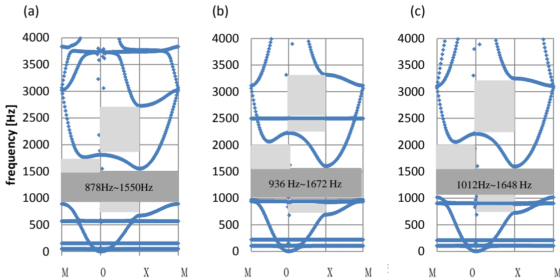
Figure 4 : Band structures of different locally resonant structures: (a) added mass is attached to the screw M3x40 at the extremity (b) added mass is attached to the screw M3x40 in the middle, (c) added mass is attached to the screw M3x25 at the extremity.
