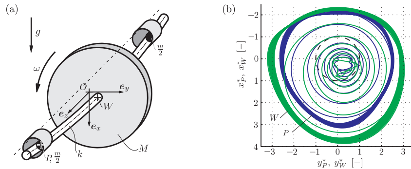
Figure 1: Model of the symmetric Lavalrotor (a), example trajectory of P and W for \omega^* > \omega_{s,lvl}^* (b)
