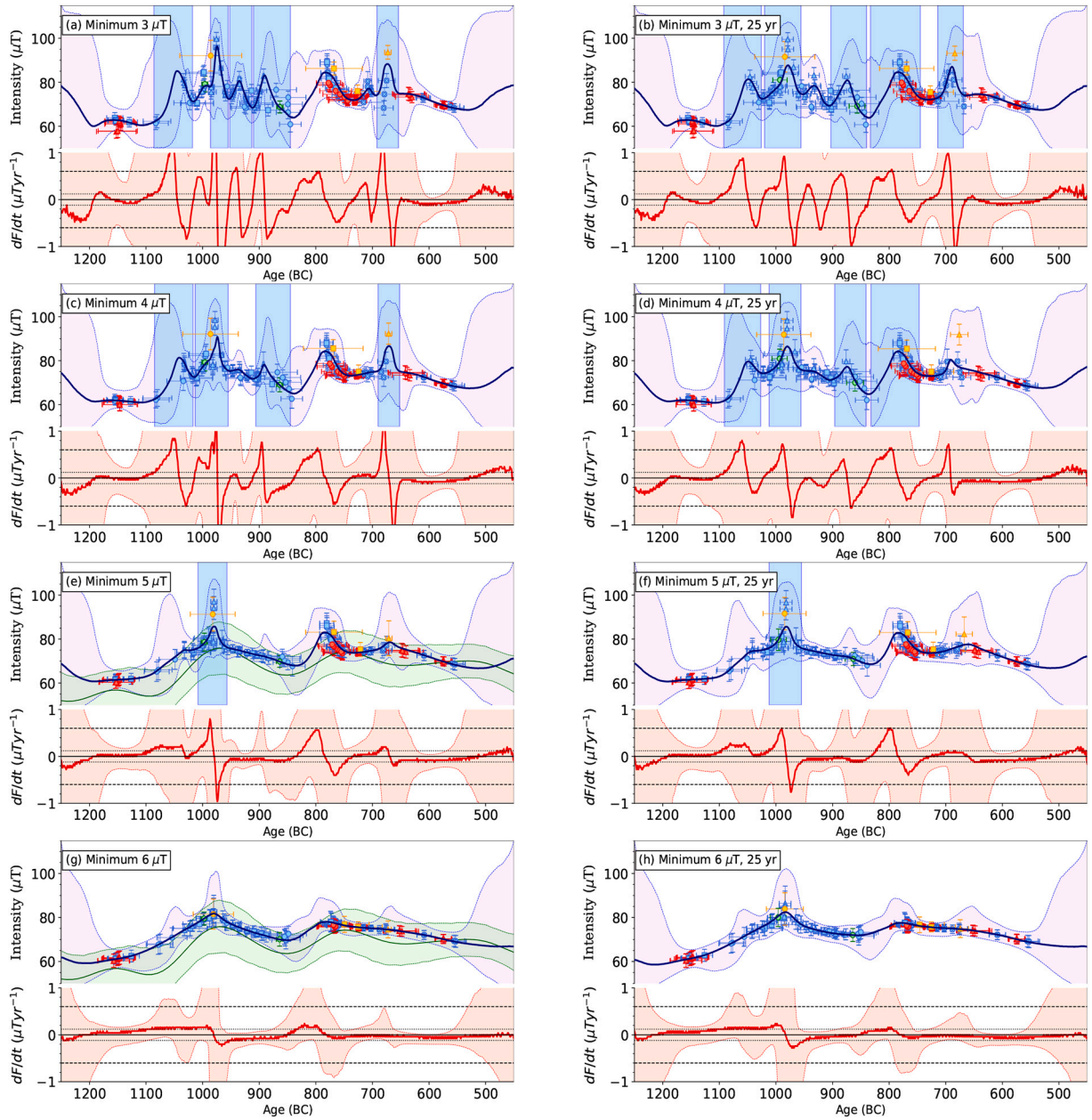
Fig. 3. The effect of a series of minimum error budgets in both intensity and age on the posterior intensity variation based on the thermal unit dataset. For each sample in the dataset, the posterior median intensity and age is plotted with the error bars showing the posterior standard deviation. Left column shows the intensity variation using the a priori ages but with a minimum intensity error of 3–6 \mu\text{T} . Right column shows the variation additionally assuming a minimum age error of 25 years. The green region in (e) and (g) shows the SHAWQ-Iron Age model with 2 standard deviations. (For interpretation of the references to colour in this figure legend, the reader is referred to the web version of this article.)
