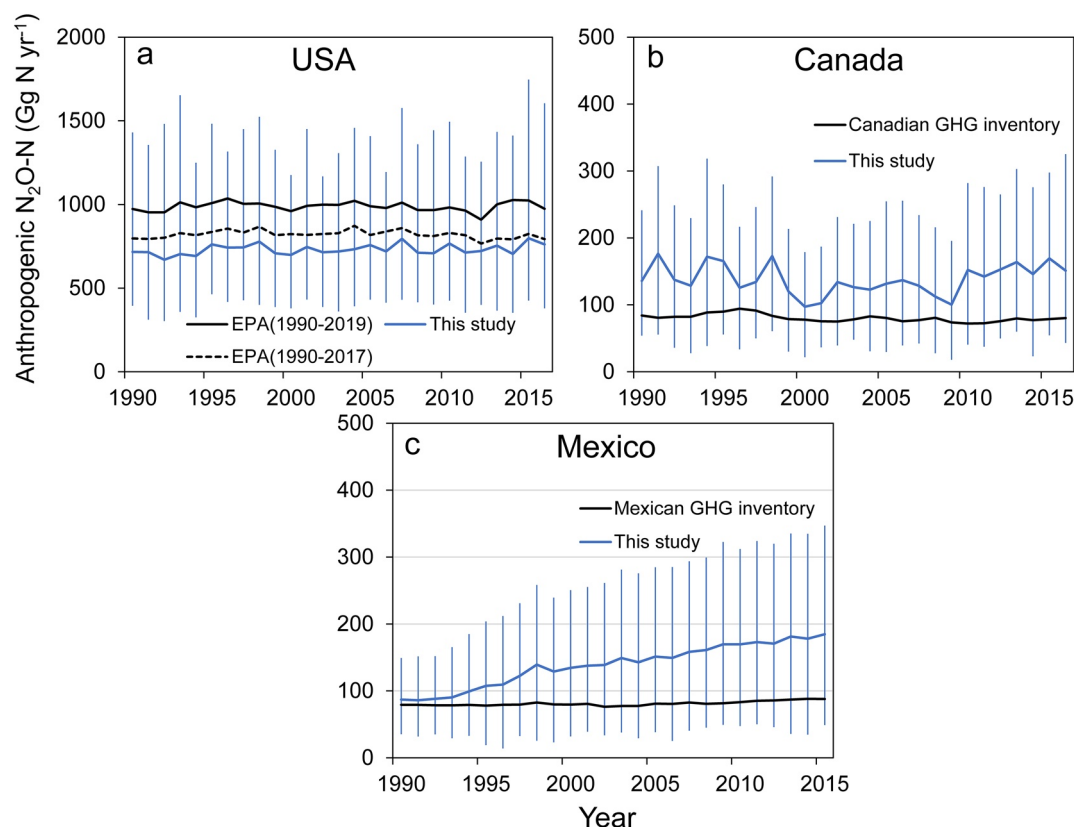
Figure 4. Comparison of our anthropogenic N 2 O emissions from BU estimates with national greenhouse gas (GHG) inventories during 1990–2016: (a) EPA; (b) Canadian GHG inventory; (c) Mexican GHG inventory. Error bars indicate the spread between the minimum and the maximum values.
