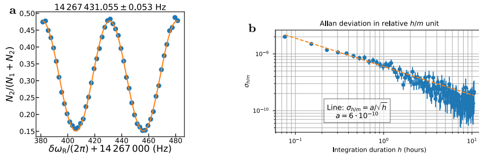
Figure 3 – a : example of spectrum : probability to be in the one output of the interferometer as a function of the Raman frequency. Each point corresponds to one realisation and takes about 1 second to acquire. b : Allan deviation of measurements taken over 48 continuous hours.
