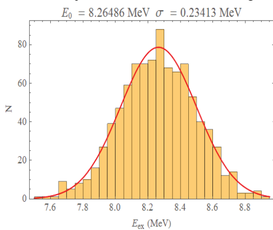
Figure 4 - Compound nucleus excitation energy reconstruction obtained from the simulation of the ^{238}\text{U}(d,d') reaction. The standard deviation of 234 keV in the excitation energy is mainly due to the detector resolution. The beam emittance considered was 0.05 mm·mrad.
