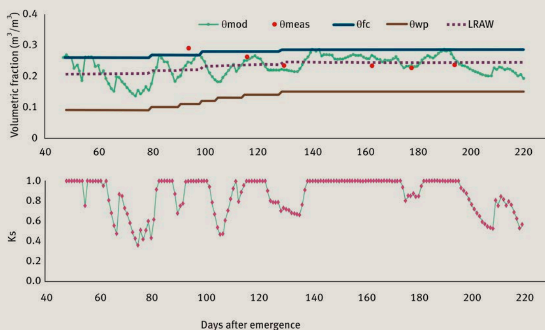
2 Seasonal course of (a, upper) soil water content expressed as volumetric fraction, either measured ( \theta_{meas} ) or modelled ( \theta_{mod} ), in relation to the lines defining the corresponding values at FC, WP and lower edge of RAW, and (b) stress coefficient estimated as in Equation 5.
