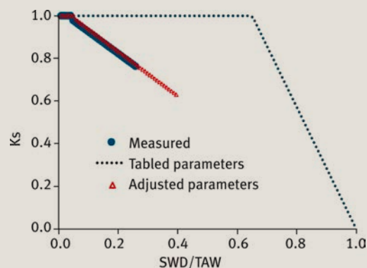
④ Relationship between K_s and SWD expressed as a fraction of TAW . Comparison between measured values and those modelled with tabled parameters (FAO 56 tabled p = 0.65 , with adjustment for ETC rates it would be 0.75) and TAW = 138 mm (derived from tabled root depth, z = 1.2 m, for ground cover of 20%, and soil parameters, assuming full colonization in horizontal). Also shown model outputs using the experimentally adjusted parameters: p = 0.04 and TAW = 310 mm.
