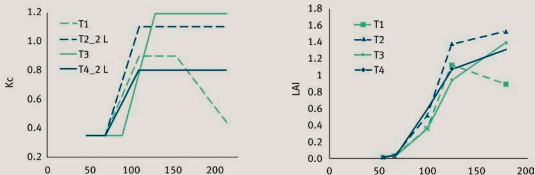
③ Seasonal course of (a, left) K_c obtained experimentally in a self-learning process from modelling and soil water content measurements, and corresponding measured LAI (b, right) for four treatments (see text): simple (T1, T3) and double line (T2 and T4), under stress (T3, T4), and without water stress (T1 and T2), for an industrial pepper crop, Portalegre (Portugal). The effect of the short term stress (Figure ②b) is excluded from these K_c values, which reflect only long term stress impact on leaf development.
