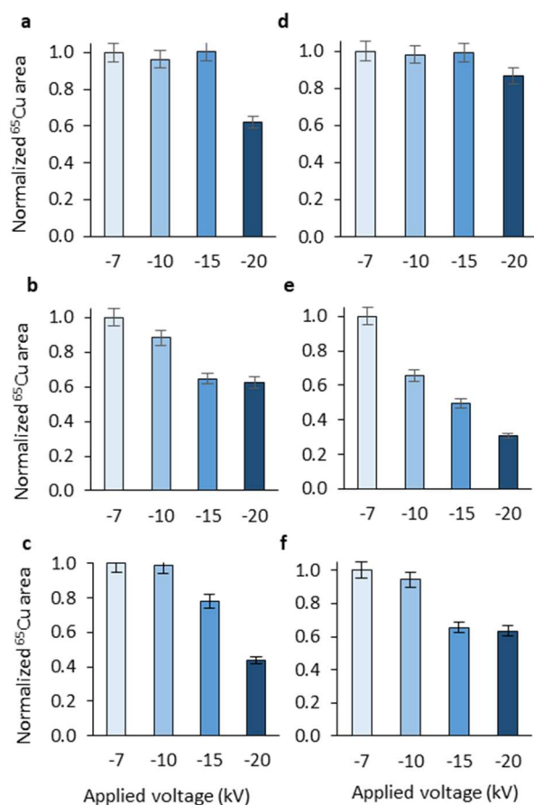
Fig. 1 Voltage effect on AB - Cu(II) (a,b,c) and on NTA - Cu(II) (d,e,f) recoveries with Tris buffer and polybrene capillary (a,d) or Tris buffer and HPC capillary (b,e) or Hepes buffer and HPC capillary (c,f) Experimental conditions: HPC or polybrene coated - capillary (75 \mu\text{m} i.d. x 64 cm), 10 mM Tris or 10 mM Hepes buffer, 15 mM NaCl at pH 7.4, 25°C. Detection: ICP-MS at m/z = 65 at the end of the capillary Separations in HPC capillary were carried out with an assisted pressure of 0.3 psi
