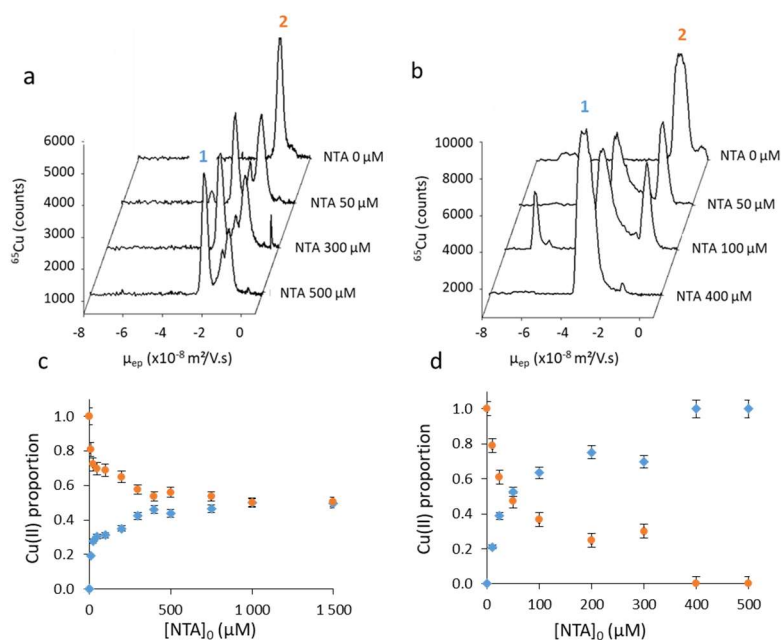
Fig. 2 Competition between A\beta_{1-16} and NTA for Cu(II) binding in Tris buffer
