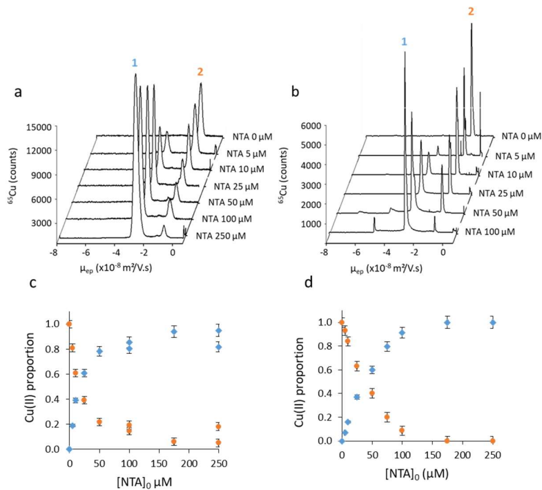
Fig.4 Competition between A\beta_{1-16} and NTA for Cu(II) binding in Hepes buffer Peaks 1 and 2 represent NTA - Cu(II) and A\beta_{1-16} - Cu(II) complexes respectively (a,b): Mobilograms obtained from CE-ICP-MS separations of 100 \mu M A\beta_{1-16} and 10 \mu M Cu(II) with various concentrations of NTA in HPC or polybrene capillary respectively (c,d): Cu(II) proportion in A\beta_{1-16} - Cu(II) ( \bullet ) or NTA - Cu(II) ( \blacklozenge ) complexes in HPC or polybrene capillary respectively as a function of NTA concentration Experimental conditions: HPC or polybrene coated - capillary (75 \mu m i.d. x 64 cm), 10 mM Hepes buffer, 15 mM NaCl at pH 7.4, 25°C. Detection: ICP-MS at m/z = 65
