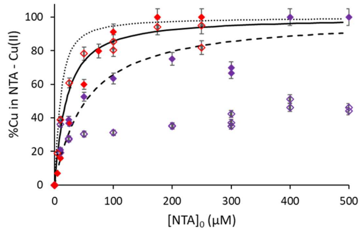
Fig.3 Experimental data for competition effect in HPC with Tris ( \diamond ), in HPC with Hepes ( \diamond ), in polybrene with Tris ( \blacklozenge ), or in polybrene with Hepes ( \blacklozenge ) and theoretical data for \log K_{A\beta_{1-16}-Cu(II)} = 9.4 (.....), \log K_{A\beta_{1-16}-Cu(II)} = 9.9 (—), and \log K_{A\beta_{1-16}-Cu(II)} = 10.4 (- - -)
