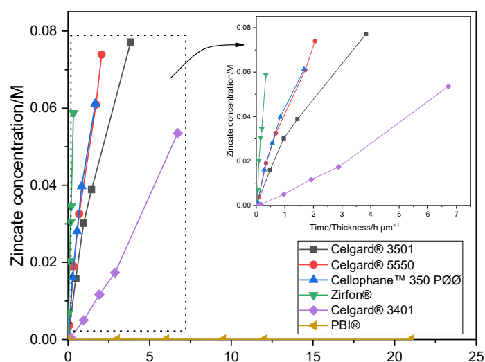
Figure 1. \text{Zn(OH)}_4^{2-} crossover concentration vs. time of Celgard® 3501, Celgard® 3401, Celgard® 5550, Cellophane™ 350 PØØ, and Zirfon® and PBI®. Lines in the figure are guides for the eye.
