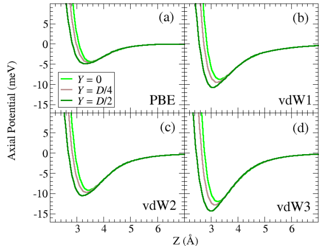
FIG. 3: (Color online) Axial potential as a function of the He-surface distance Z for fixed values of the coordinate Y across the \langle 100 \rangle channel. Different exchange-correlation functionals are considered in each panel: (a) PBE, (b) vdW1, (c) vdW2, and (d) vdW3 (See text for the labeling of vdW approaches).
