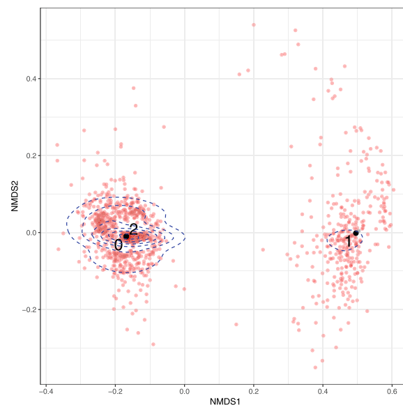
Fig. 9 Comparison of Nanopore reads to STRONG prediction for COG0532 from Bin_72. Non-metric multidimensional scaling of Nanopore reads that mapped to COG0532 from Bin_72 of the anaerobic digester time series (red) together with the three haplotypes reconstructed from short reads by STRONG (black 0, 1 and 2). Haplotypes 0 and 2 were identical for COG0532. Distances were calculated as fractional Hamming distances (see text) on short read variant positions (see “Methods - Nanopore sequence analysis” section). Blue dashed lines indicate read density contours
