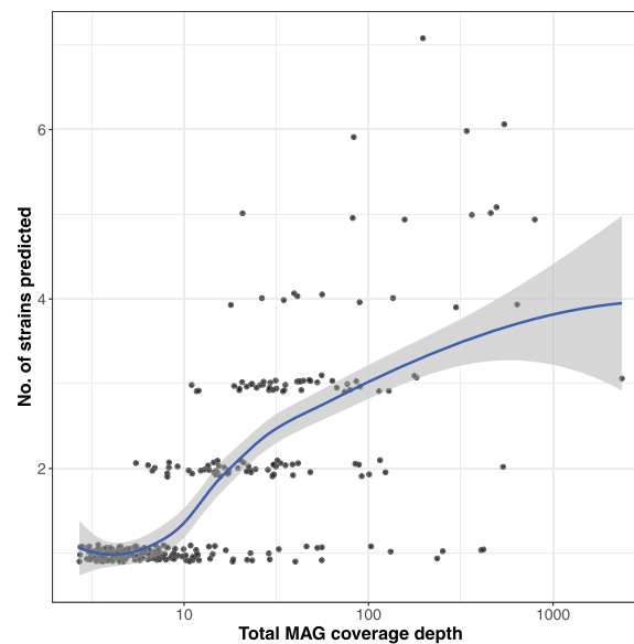
Fig. 7 Number of strains resolved by STRONG against MAG coverage depth for the AD time series. Pearson's correlation between coverage depth and number of strains ( r = 0.36 , p = 1.004e - 10 ). The curve indicates a LOESS smoothing
