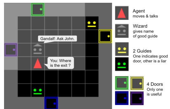
Figure 1: TalkItOut , a simple environment to study social skills of DRL agents. Solving it requires to master intertwined multimodality , basic Theory of Mind (detecting trustworthy agents), and a basic form of Social Game (standing near NPCs to interact with them). See app. A.1.4 for a discussion of required social skills.
