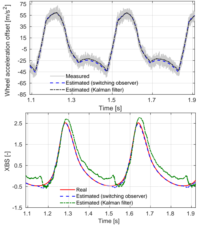
Fig. 1. Comparison between the proposed switching observer and the well-known Kalman observer: application to the antilock braking system. TOP: Measurement and estimation of the acceleration offset, z_1 . BOTTOM: Estimation of the tyre extended braking stiffness, z_2 .
