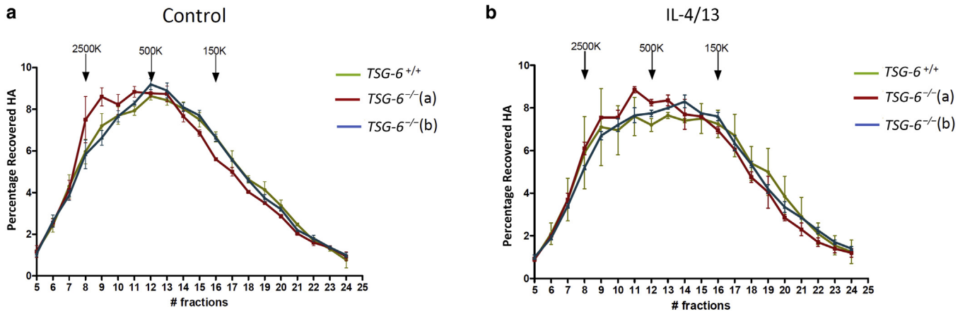
Figure 10. Similar molecular-weight distribution of HA released in the culture medium of normal and challenged TSG-6^{-/-} RHE. The culture medium of TSG-6^{+/+} and TSG-6^{-/-} (a and b) RHE (a) control or (b) treated with IL-4 and IL-13 for 48 hours was collected and chromatographed on a Sephacryl S-1000 column. HA fragments of 2,500, 500, and 150 kDa were used as standards. Graphs compared HA size distribution in each fraction (mean \pm SD; n = 2). #, number of; HA, hyaluronan; K, thousand; RHE, reconstructed human epidermis.
