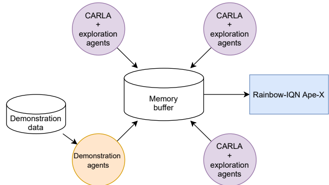
Fig. 3: Simplified representation of the distributed GRIAD setup with a Rainbow-IQN Ape-X backbone. A central computer receives data in a shared replay buffer from both exploration and demonstration agents running on other computers. Data are sampled from this replay buffer to make the backpropagation and update the weights of all the agents. Images from the agents are encoded using the network presented in Fig. 2 before being stored in the memory buffer.
