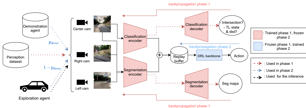
Figure 1. General Reinforced Imitation (GRI) is applied to visual-based autonomous driving in an end-to-end pipeline composed of a perception module encoding RGB images from the three cameras on the driving agent and a decision-making module inferring an action from the encoded features. This pipeline is trained in two phases: (1) Visual encoders are pretrained on a perception dataset on several auxiliary tasks, which are semantic segmentation, road type classification, relevant traffic light presence, and if there is such a traffic light, its state and the distance to it. (2) Visual encoders are frozen and a GRI-based DRL network is trained with both pre-generated expert data with an offline demonstration agent and an online exploration agent gathering data from a simulator. At any given training step, the next episode to add to the replay buffer comes from the demonstration agent with a probability of p_{demo} , else from the exploration agent. Actions correspond to a pair (steering, throttle) to apply to the car.
