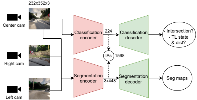
Figure 2. Feature extraction from RGB camera images for the visual subsystem. Two encoder-decoder networks are pretrained on segmentation, classifications and regression tasks. Classifications and regression are only performed on the center image while all three images are segmented. After training, the visual encoders serve as fixed feature extractors with frozen weights. For the DRL backbone training, both encoder outputs are concatenated and sent to the memory buffer as input to DRL. Both encoders are Efficientnet-b1. The segmentation decoder is fully convolutional, and the classification decoder is an MLP with several outputs.
