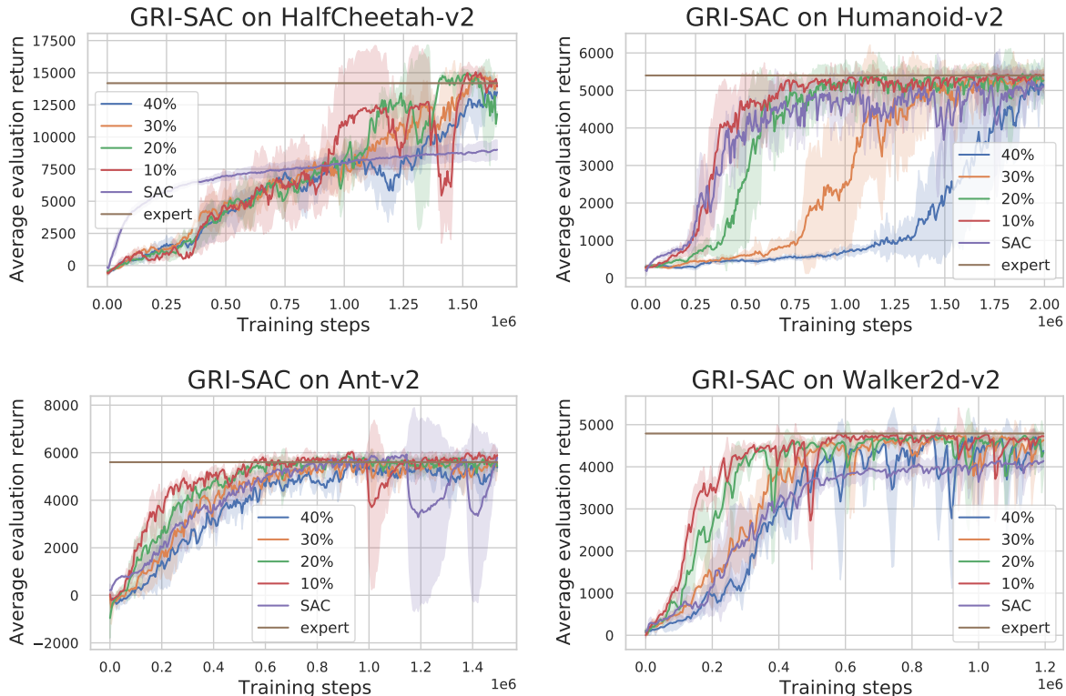
Figure 5. Evolution of the evaluation reward on Mujoco environments with different proportions of demonstration agents with GRI-SAC. GRI-SAC with 0% demonstration agent is vanilla SAC. We observe that GRI-SAC always reaches the level of the expert even when the expert is significantly better than the trained vanilla SAC. The proportion of demonstration agent have a significant impact on the dynamic of the convergence.
