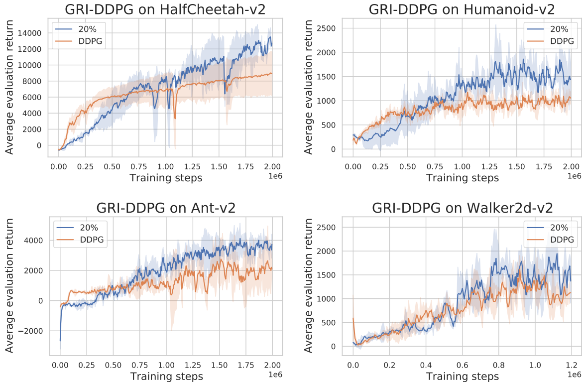
Figure 6. Comparison of the evaluation reward evolution on Mujoco environments between GRI-DDPG with 20% of demonstration agents and vanilla DDPG. GRI-DDPG systematically leads to a better reward than vanilla DDPG. However, contrarily to GRI-SAC, GRI-DDPG with 20% demonstration agents does not systematically reach the expert level.
