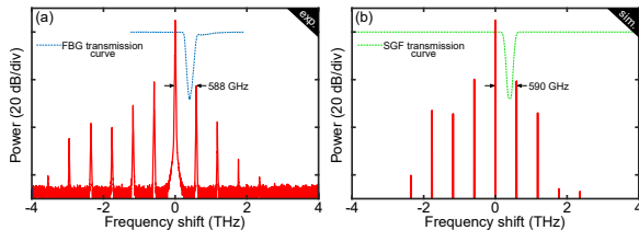
Fig. 1: OFC generated in experiment a) and in numerical simulations b). Dotted blue and green lines in a) and b) denote filter transmission profiles.
