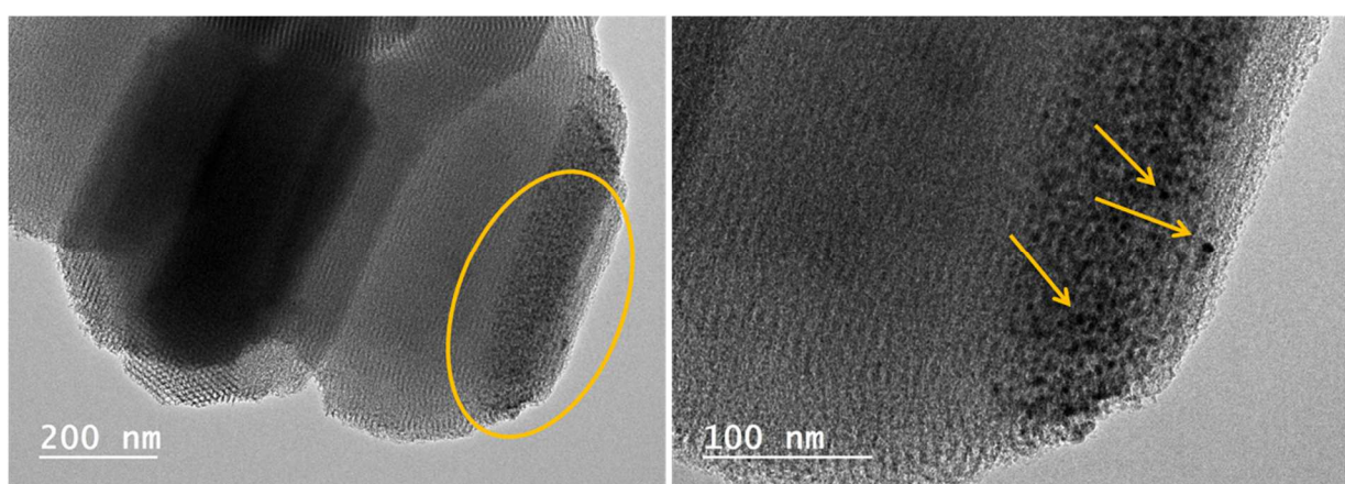
Fig. 4 TEM images of Cu/SBA-15-Coffee ( a ) and Cu/SBA-15-Tea ( b )
