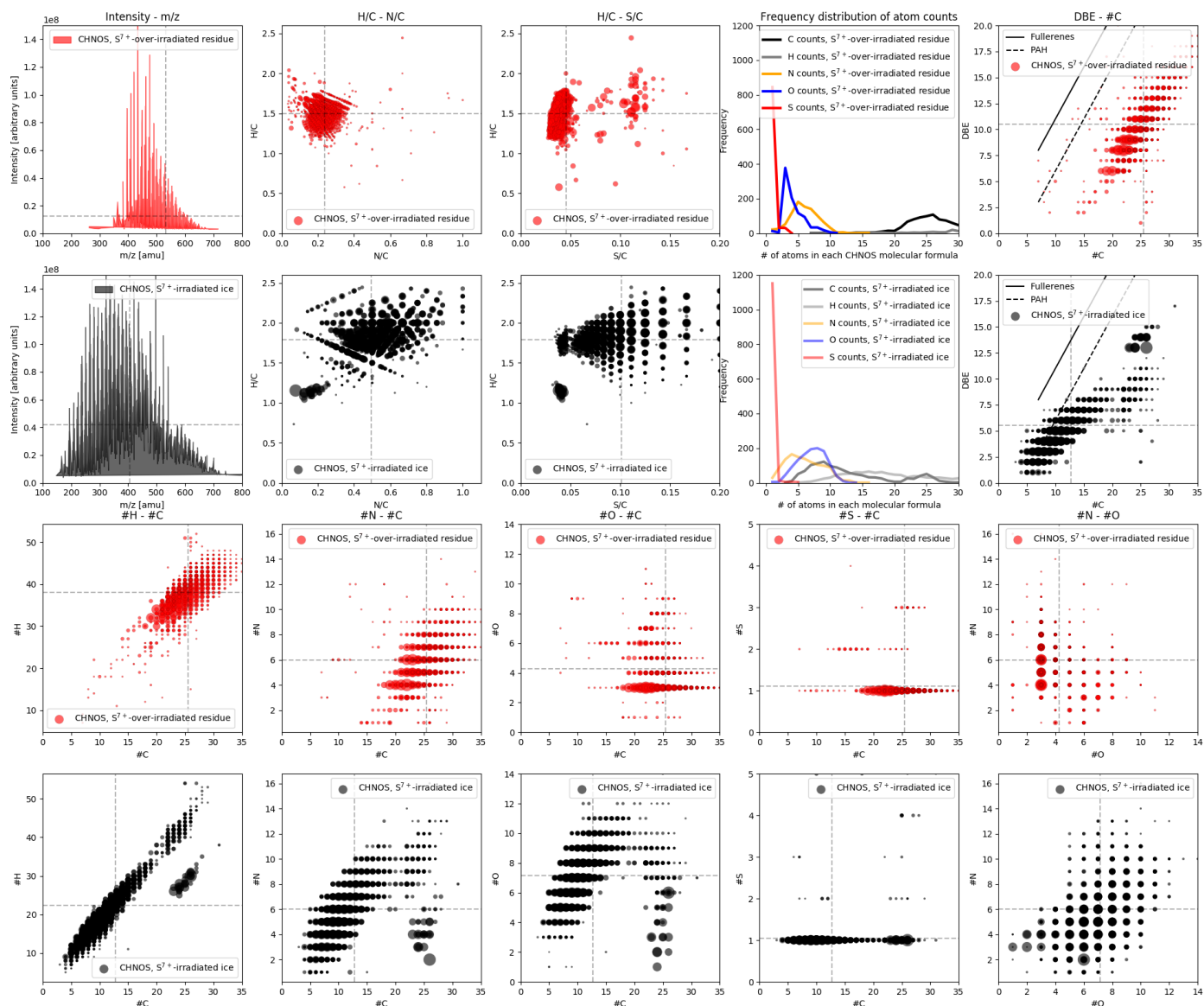
Fig. B.3. Characteristics of CHNOS compounds formed on residues (red, 1st and 3r row) or inside ices (black, 2nd and 4th row) - detailed plots. 1st-2nd row, from left to right: Intensity- m/z , H/C-N/C, H/C-S/C plots, frequency distribution of atom counts, DBE-#C plot. 3rd/4th row; from left to right: #H-#C, #N-#C, #O-#C, #S-#C and #N-#O plots. Dashed lines represent mean values.
