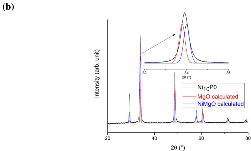
FIGURE S2. (a) Profile of refinement for the Ni 10 P0 sample. (b) Calculated diffractograms for MgO and NiMgO, together with the real diffractogram for Ni 10 P0 performed with synchrotron radiation (10 keV).
