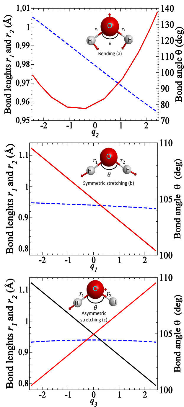
Figure 2. Normal modes of H 2 O. The figure shows the dependence of inter-particle distances r_1 , r_2 and the bond angle \theta as functions of normal mode coordinates: (a) bending, (b) symmetric stretching and (c) asymmetric stretching. The arrows indicate the direction and magnitude of displacements for each mode. Bond lengths are given with solid lines with values on the left axis, while the bond angle is given with a dashed line with values on the right axis of each panel. Note that the curves of the bond lengths r_1 (black) and r_2 (red) are indistinguishable for the bending and symmetric stretching modes.
