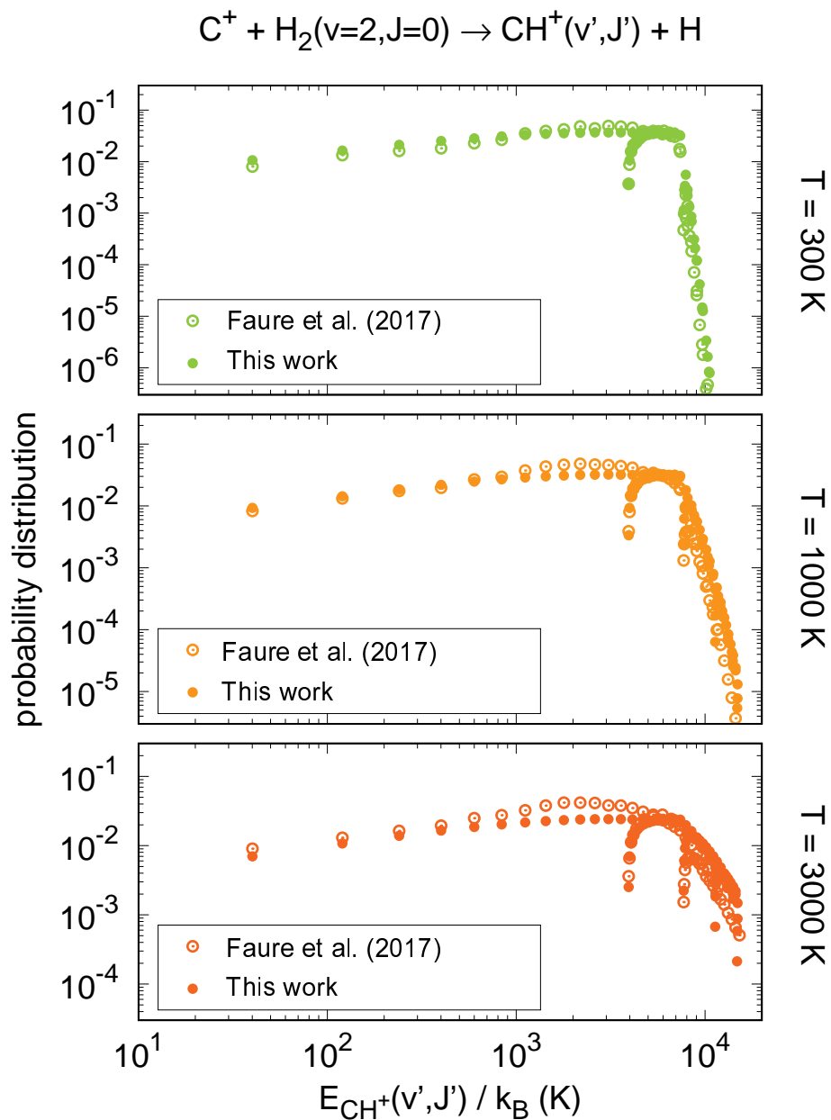
Figure 15. Probability distributions of forming CH^+ in its rovibrational levels (v', J') through the reaction of C^+ with H_2(v = 2, J = 0) as function of the level energy E_{CH^+(v', J')} . The distributions computed with equation B5 (filled circles) are compared with those obtained by F17 (empty circles) for a kinetic temperature of 300 K (top panel), 1000 K (middle panel), and 3000 K (bottom panel).
