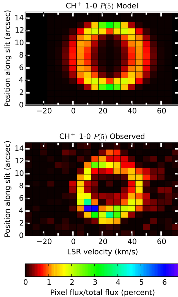
Figure 11. Top panel: Specific intensity of the 1 - 0 P(5) line of \text{CH}^+ computed using an isochoric PDR model with n_{\text{H}} = 3 \times 10^5 \text{ cm}^{-3} wrapped around a sphere expanding at a velocity V_{\text{exp}} = 20 \text{ km s}^{-1} as a function of the velocity and the position along a slit identical to the observational setup. Intensities are averaged over a spatial bin of 1'' and a spectral bin of 5 \text{ km s}^{-1} as in Figures 2 – 4. The source was assumed to have a centroid v_{\text{LSR}} of 25 \text{ km s}^{-1} with its center at +8'' . Bottom panel: observed PV diagram for \text{CH}^+ 1 - 0 P(5)
