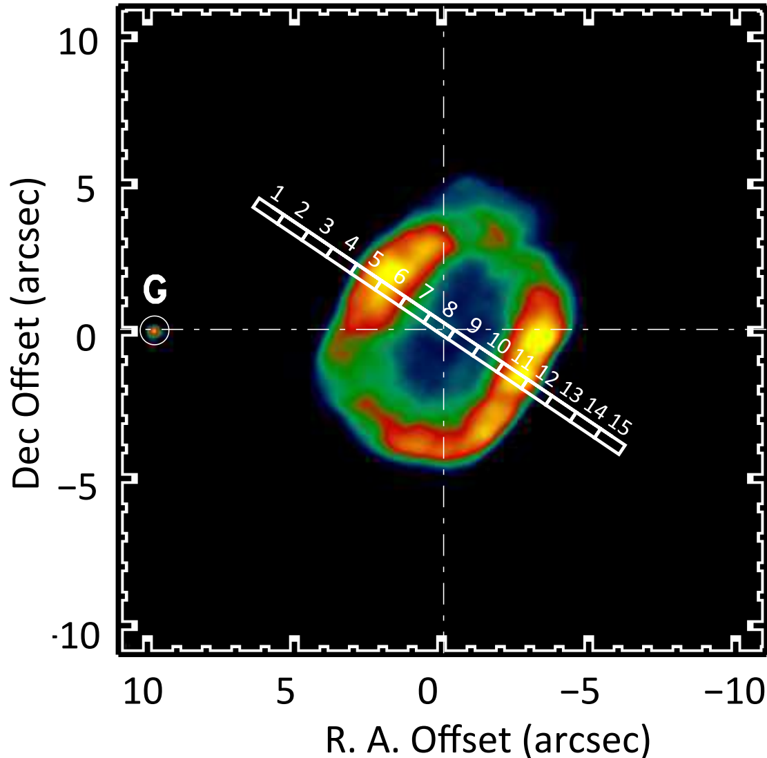
Figure 1. K -band image of NGC 7027, obtained with the slit viewing camera. White boxes indicate the aperture extraction regions adopted, with the numbering system used in the text. The R.A. and Dec. offsets are given relative to the central star at \alpha = 21^{\text{h}} 07^{\text{m}} 1^{\text{s}}.793 , \delta = 42^{\circ} 14' 9''.79 (J2000). “G” indicates the star used for guiding.
