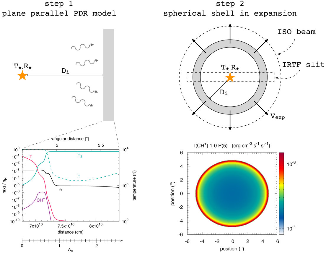
Figure 9. Summary of the modeling strategy. Top left : the thermochemical and excitation profiles of a neutral slab of gas illuminated on one side by a star are calculated in a plane parallel geometry. Bottom left : kinetic temperature T and abundances of \text{H} , \text{H}_2 , e^- , and \text{CH}^+ obtained for an isochoric PDR with a density n_{\text{H}} = 3 \times 10^5 \text{ cm}^{-3} as functions of the distance to the star, starting from the ionization front. (Results for a isochoric PDR with this density, obtained from the earlier model of GC13, are shown in their Figure 6.) Top right : the radiative transfer within the rovibrational lines of \text{H}_2 and \text{CH}^+ is computed by wrapping the PDR around a sphere of radius D_i expanding at a constant velocity V_{\text{exp}} . Bottom right : example of the intensity map obtained for the 1 - 0 \text{ P}(5) line of \text{CH}^+ .
