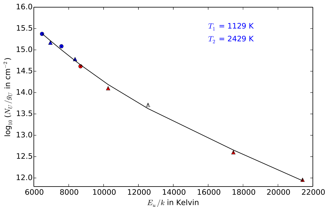
Figure 8. H _2 rotational diagram. Red, blue and white symbols refer to states with v = 0, 1 and 2 respectively; triangles represent states of ortho-H _2 (i.e. with J_U odd) and circles represent states of para-H _2 ( J_U even); the black line is a two-component fit.
