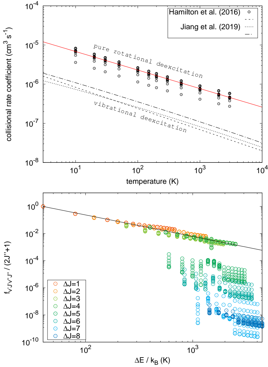
Figure 14. Top: total collisional deexcitation rate coefficients for \text{CH}^+ in collisions with e^- . Open circles correspond to deexcitation of pure rotational levels (Hamilton et al. 2016). Black curves correspond to vibrational deexcitation of the v' = 1 (dashed), v' = 2 (dotted), and v' = 3 (dotted-dashed) levels of \text{CH}^+ (Jiang et al. 2019). The red curve shows a fit of pure rotational data using Eq. B3 with \alpha = -4.7 , \beta = -0.47 , and \gamma = 0 . Bottom: probability distribution of rotational deexcitation as function of the level energy difference \Delta E and \Delta J (Hamilton et al. 2016). The black curve indicates the power-law fit used in Eq. B4.
