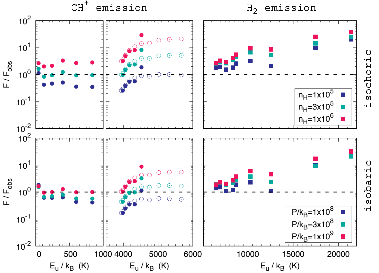
Figure 10. Ratios of predicted to observed fluxes F/F_{\text{obs}} computed for the pure rotational lines of CH + (left panel), the rovibrational lines of CH + (middle panel), and the rovibrational lines of H 2 (right panel) as functions of the energies E_u/k_B of the upper levels of the transitions. The models include isochoic PDRs (top panels) with n_{\text{H}} = 10^5 , 3 \times 10^5 , and 10^6 cm -3 and isobaric PDRs (bottom panels) with P/k_B = 10^8 , 3 \times 10^8 , and 10^9 K cm -3 . R-branches and P-branches are shown with filled and empty circles, respectively. Simulated fluxes are obtained by integrating the line intensities over the instrumental beam (see text for details).
