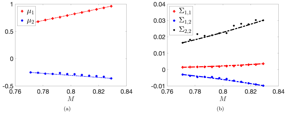
Figure 12: transonic flow past an airfoil. Behavior of the MLE estimates \mu_{\text{mle}} and \Sigma_{\text{mle}} (18) with respect to the Mach number.
