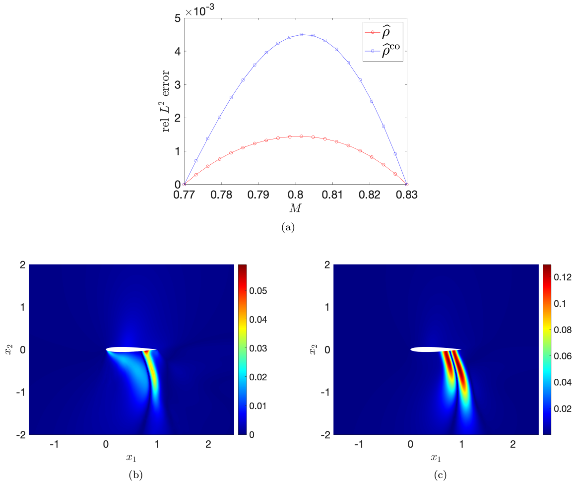
Figure 15: boundary-aware transportation of Gaussian models (angle of attack 4^\circ ). (a) behavior of the relative L^2 error for BA convex displacement interpolation. b)-(c) behavior of the error fields |\hat{\rho}(s, x) - \rho(x; M)| and |\hat{\rho}^{\text{co}}(s, x) - \rho(x; M)| for M = 0.8 and s = 0.5 .
