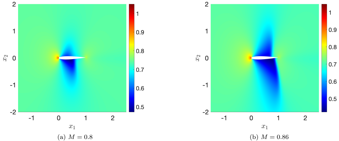
Figure 17: transonic flow past an airfoil at angle of attack 1^\circ . Flow density for two values of the Mach number.
