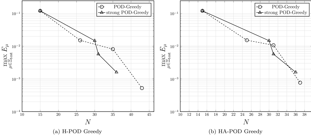
Figure 9: Out-of-sample performance of the ROM parametric problem obtained using the POD-Greedy algorithm. Comparison with strong POD Greedy.
