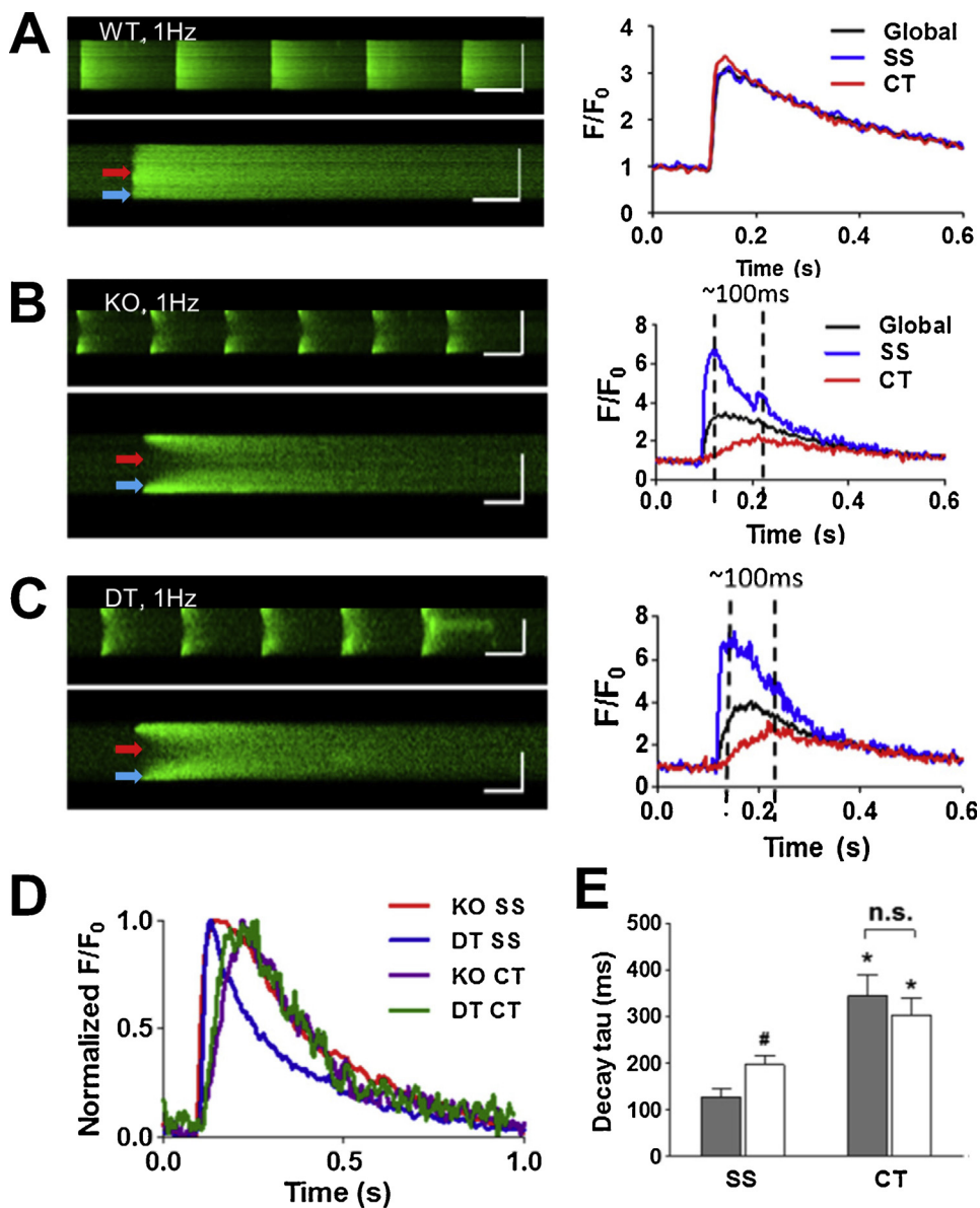
Fig. 4. Ca release in control and NCX1 KO atrial myocytes. A. Left, Confocal line-scan images of five Ca transients (CaT) from a representative atrial myocyte loaded with Fluo-4-AM and field stimulated at 1 Hz (upper image), and a single CaT taken from the same cell but shown on an expanded time scale (lower image). Horizontal scale bars represent 500 ms (upper panel) and 100 ms (lower panel), while vertical scale bars represent 10 \mu\text{m} for both images. Right, fluo-4 fluorescence intensity ( F/F_0 ) plots over time from the cell in A, at 1.5 \mu\text{m} from the subsarcolemmal space (SS, blue) or in the cell center (CT, red). Color coded arrows on the image correspond to the locations where the fluorescence was sampled for intensity plots. The global CaT is shown in black. Note the typical synchronous Ca release and uptake at both locations (with the global trace overlapping the SS and CT traces). B. Left, representative line-scan images collected as in A, but for an NCX1 KO atrial myocyte. Note the dramatically different kinetics of the SS (directly triggered) versus CT (propagated) locations. C. Similar to A and B but in a detubulated (DT) WT myocyte. D. Normalized, field stimulation-induced intracellular CaTs from representative DT and NCX1 KO myocytes at the SS regions (DT, blue; NCX1 KO, red), as well as the CT regions (DT, green; NCX1 KO, purple). E. Summary plot of the local CaT decay tau from SS and CT regions in DT (grey) and KO (white) atrial myocytes. * P < 0.05 , CT vs. SS, # P < 0.05 , KO vs. DT, unpaired Student's t-test, n = 9 cells from 3 animals for DT, n = 27 cells from 6 animals for KO. Note the slowed decay in the SS region of NCX1 KO compared to DT. Modified from Yue et al, 2017 [46].
