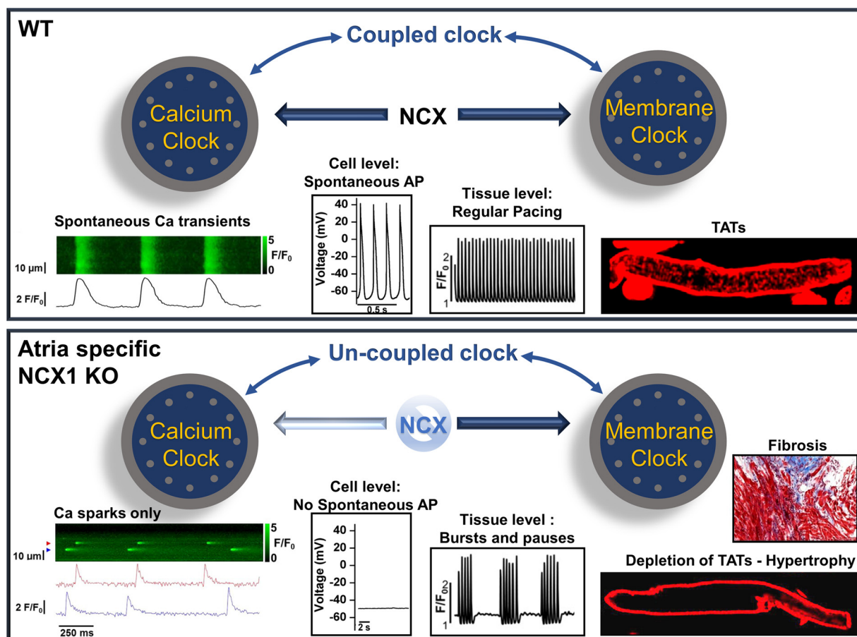
Fig. 5. Summary comparison of SAN function in WT versus NCX1 KO. In WT mice (upper panel), a calcium clock based on NCX1 activation by LCRs depolarizes the membrane at rhythmic intervals, which leads to a large Ca transient. This in turn generates regular action potentials both at the cell and tissue level. In addition, extensive TATs contribute to the microdomain co-localization between LCRs and the membrane. In the KO, the absence of NCX1 disengages the link between the Ca clock and membrane depolarization, illustrated by normal LCRs but no calcium transient or spontaneous action potentials. Ablation of NCX1 also promotes remodeling characterized by loss of TATs, hypertrophy and fibrosis.
