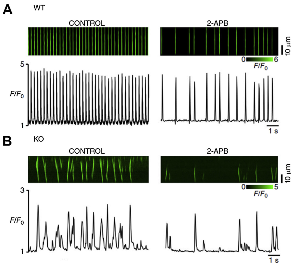
Fig. 2. Ca oscillations in WT and NCX1KO SAN cells loaded with fluo-4: involvement of IP 3 Receptors. A-B. Confocal linescan images and corresponding fluorescence intensity plots of representative WT (A) and NCX1 KO (B) SAN cells before (CONTROL) and after superfusion with the IP 3 antagonist 2-APB (2 μM). Note that both spontaneous action potential-mediated Ca transients (in WT) and Ca waves (in KO) slow in response to 2-APB, consistent with modulation of the Ca clock by IP 3 receptors. Modified from Kapoor et al, 2015 [30].
