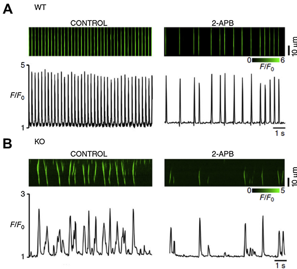
Fig. 2. Ca oscillations in WT and NCX1KO SAN cells loaded with fluo-4: involvement of \text{IP}_3 Receptors. A-B. Confocal linescan images and corresponding fluorescence intensity plots of representative WT (A) and NCX1 KO (B) SAN cells before (CONTROL) and after superfusion with the \text{IP}_3 antagonist 2-APB (2 \mu\text{M} ). Note that both spontaneous action potential-mediated Ca transients (in WT) and Ca waves (in KO) slow in response to 2-APB, consistent with modulation of the Ca clock by \text{IP}_3 receptors. Modified from Kapoor et al, 2015 [30].
