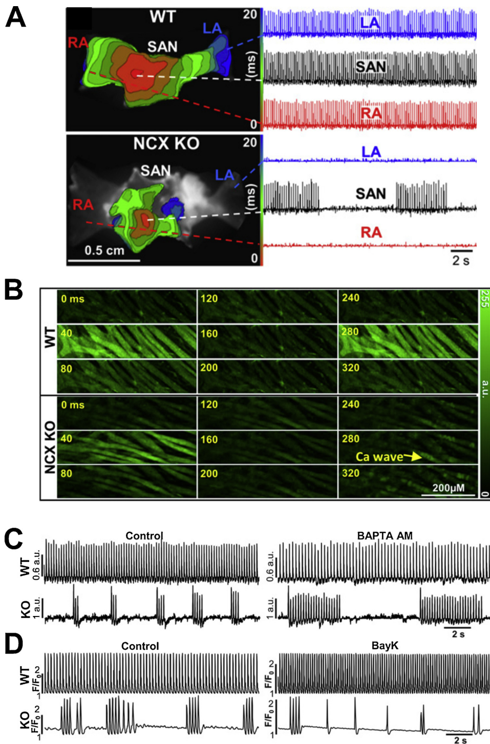
Fig. 3. Optical voltage mapping of explanted SAN/atrial tissue and Ca dynamics in the intact SAN tissue. A. Isochronal voltage maps from WT and NCX1 KO tissue (Left) and corresponding optical recordings of APs from discreet locations (Right). B. Time series of 2D confocal images of Ca [Cal-520 fluorescence in arbitrary units (a.u.); 50-Hz acquisition speed] in WT and NCX1 KO SANs. C. Optical recordings of spontaneous APs in WT (Upper) and NCX1 KO (Lower) SAN tissue, before (Left) and after (Right) incubation with BAPTA AM (2 \mu M). D. Confocal recordings of Ca transients in WT (Upper) and NCX1 KO (Lower) SAN tissue, before (Left) and after (Right) perfusion with BayK (1 \mu M). Modified from Torrente et al, 2015 [33].
