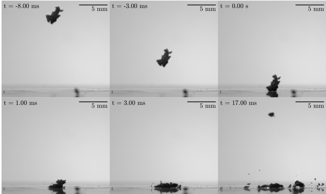
Fig. 3 Example images of a snowflake recorded with camera 1 (front view) having a resolution of 24.1 \mu\text{m}/\text{pixel} . The snowflake's maximum dimension is 3.5 mm and its terminal velocity is 1.36 m/s.
