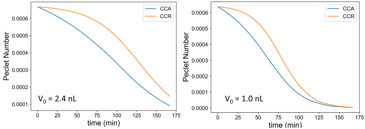
Figure F. Evolution of Peclet number for CCA and CCR models corresponding to the experimental condition described in Figure 4b. (If Peclet number \ll 1 , the microdroplet is considered to have homogeneous composition)
