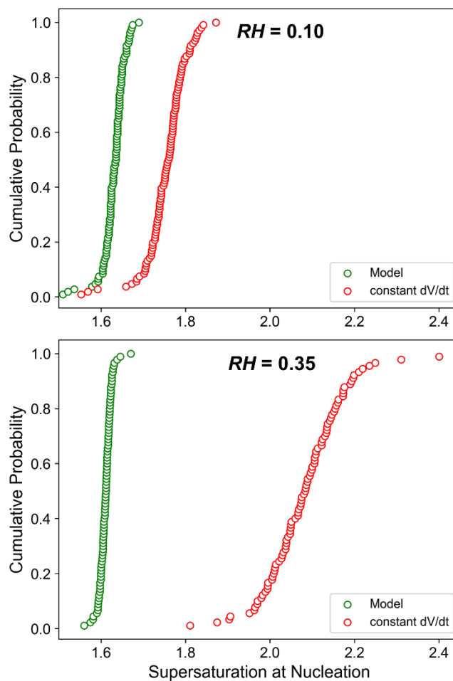
Figure H. Cumulative probability distribution of supersaturation at nucleation S_n for microdroplets at identical experimental configuration ( V_0 = 55 \text{ pL} , S_0 = 0.70 , L_1/R_0=5.6 , L_2/R_0=32 ) but at different hygrometric conditions.
