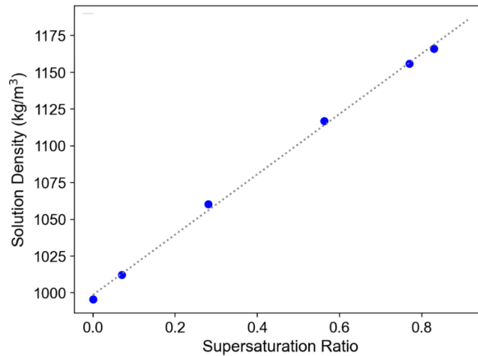
Figure B. Variation of aqueous NaCl density as a function of supersaturation ratio. 6 The
