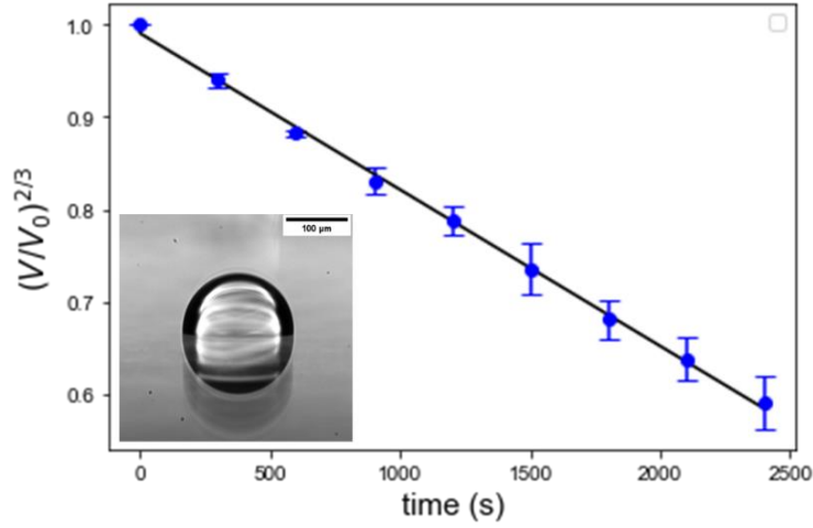
Figure E. Plot of (V/V_0)^{2/3} vs time. From the slope, the diffusivity of water in PDMS oil can be determined using equation S34, from which we obtained D = 6.74 \times 10^{-9} \text{ m}^2 \text{ s}^{-1} .
