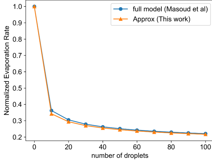
Figure D. Comparison of the full model (Masoud et al, equation S23) for the middle droplet against our approximation (equation S26).
