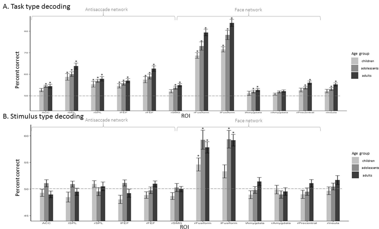
Figure 5. ROI-based MVPA: mean percentage decoding accuracy in children, adolescents, and adults. SVM classification accuracy for saccade category (task) detection was averaged per age-group per region. Statistical significance was assessed with 1-sample t-test against 50% chance and corrected for multiple comparisons using the FDR method. Above chance statistical significance ( P < 0.05 ) is represented by *. Significant differences between groups of P < 0.05 are represented by *. (A) Saccade type (task) decoding. (B) Stimulus type (category) decoding.
