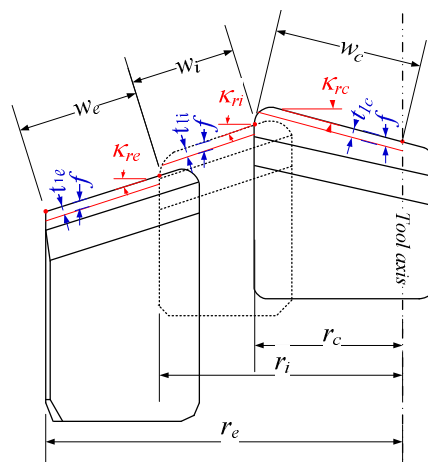
FIG. 2 – Engaged cutting edge width ( w ) and undeformed chip thickness ( t_1 ) of each insert of the BTA deep hole drilling tool.
