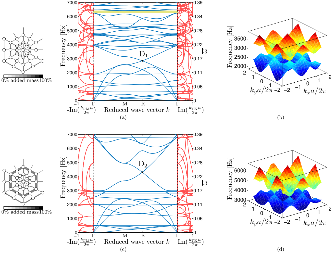
Figure 12: Band diagrams, corresponding unit cells, and dispersion surfaces computed for the generated Dirac cones obtained using the optimization objectives \varphi_n^{(D)} (Eq. (11)) for n = 10 and n = 17 , respectively : D_1 (2839 Hz) with its (a) band diagram, unit cell, (b) and dispersion surface and D_2 (4298 Hz) with its (c) band diagram, unit cell, and (d) dispersion surface.
