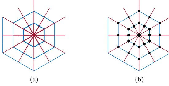
Figure 3: Design options used for parameter optimization: (a) variation of radial and viscid thread diameters and (b) introduction of localized masses at the junctions of threads.
