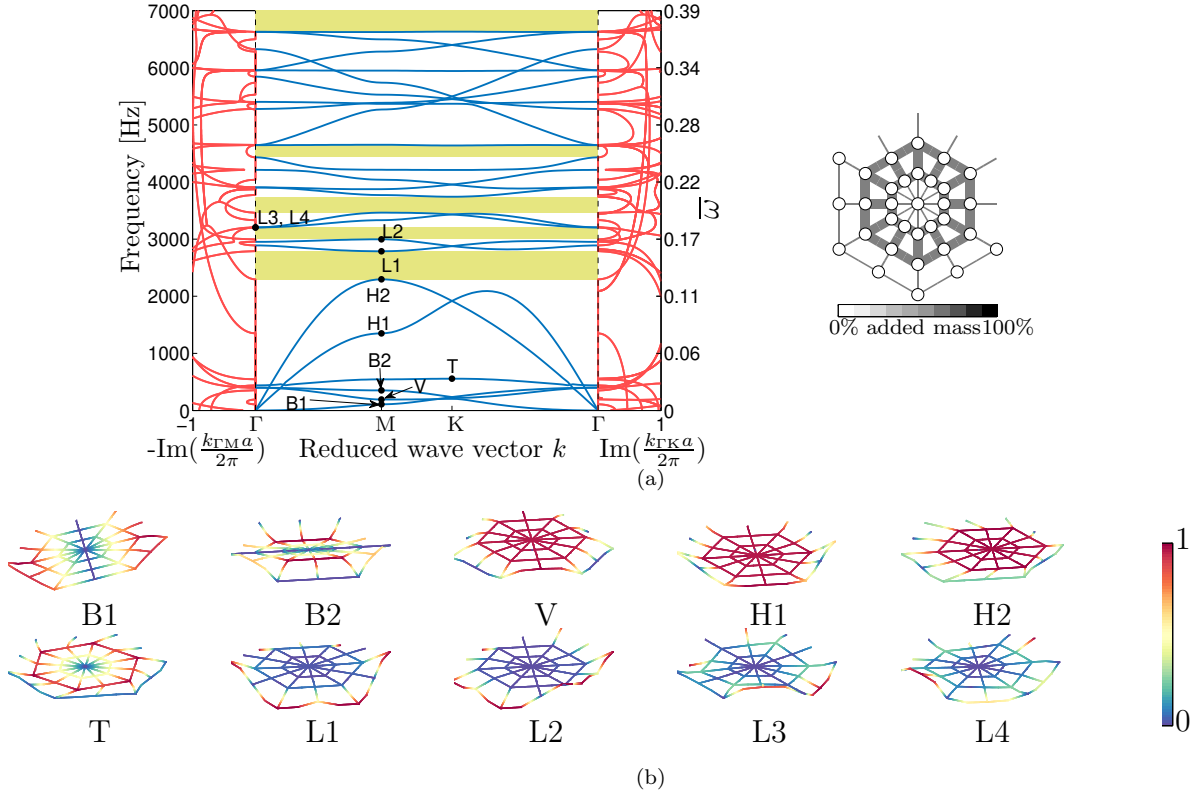
Figure 5: Results for optimized structure for maximum normalized BG width between 6th and 7th bands: (a) band diagram with BGs between 2296 Hz – 2788 Hz, 2998 Hz – 3025 Hz, 3464 Hz – 3742 Hz, 4433 Hz – 4640 Hz, and 6633 Hz – 7000 Hz and its corresponding unit cell obtained using optimization objective \varphi_6^{(s)} (Eq. (7)). (b) Wave modes are separated between low-frequency (B1, B2, V, H1, H2, and T, dominated by rigid-body-like inclusion behavior) and mid- to high-frequency wave modes (L1, L2, L3, and L4) with localized motion at the outer threads.
