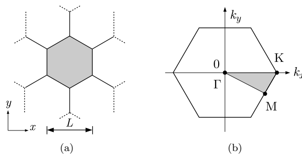
Figure 2: (a) Two-dimensional hexagonal periodic medium with a highlighted unit cell and (b) FBZ with its highlighted IBZ and high symmetry points \Gamma (0,0), M ( \pi/L , -\pi/L\sqrt{3} ), and K ( 4\pi/3L , 0).
