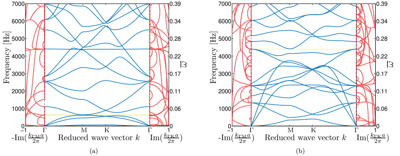
Figure 7: Band diagrams of structures with added masses: (a) concentrated at the PC center (BG around 630 Hz) and (b) distributed around the first junctions around PC center (BG around 4410 Hz).
