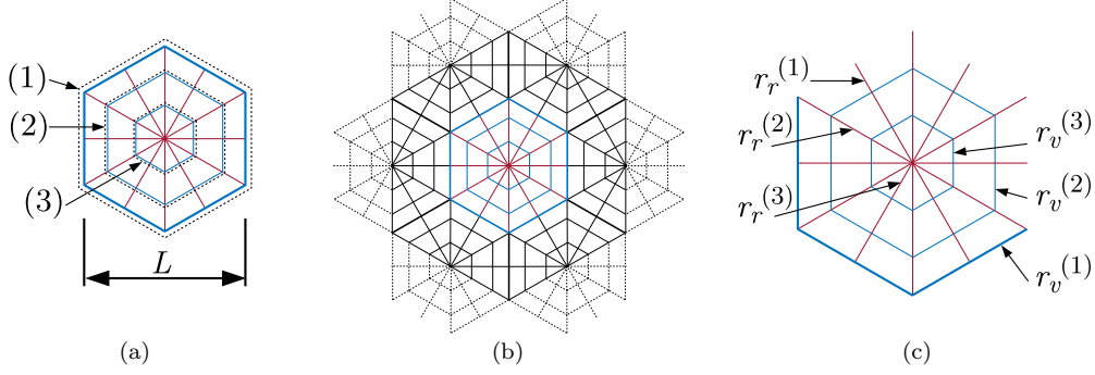
Figure 1: Spider web-inspired periodic frame: (a) single hexagonal frame structure (radial threads indicated as red lines and viscid threads indicated as blue lines) with distinct composing layers, (b) periodic structure obtained from the repetition of the spider web-inspired frame (colored) in a hexagonal lattice, (c) representative unit cell used to obtain the periodic structure (some frame elements are removed at the edges of the unit cell so they are not duplicated in the corresponding periodic structure).
