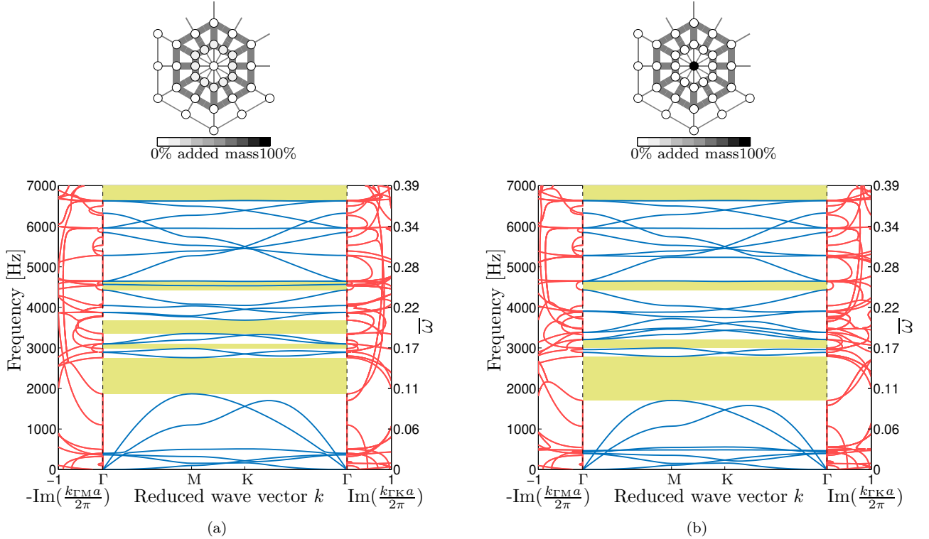
Figure 8: Band diagrams computed (considering a previously optimized threads configuration) using a mass distribution for maximizing the normalized BG width between (a) the 6th and 7th bands (first BG between 1868 Hz – 2759 Hz) and (b) the 7th and 8th bands (first BG between 1705 Hz – 2788 Hz) and their corresponding unit cells obtained using optimization objectives \varphi_n^{(s)} (Eq. (7)) for n = 6 and n = 7 , respectively.
