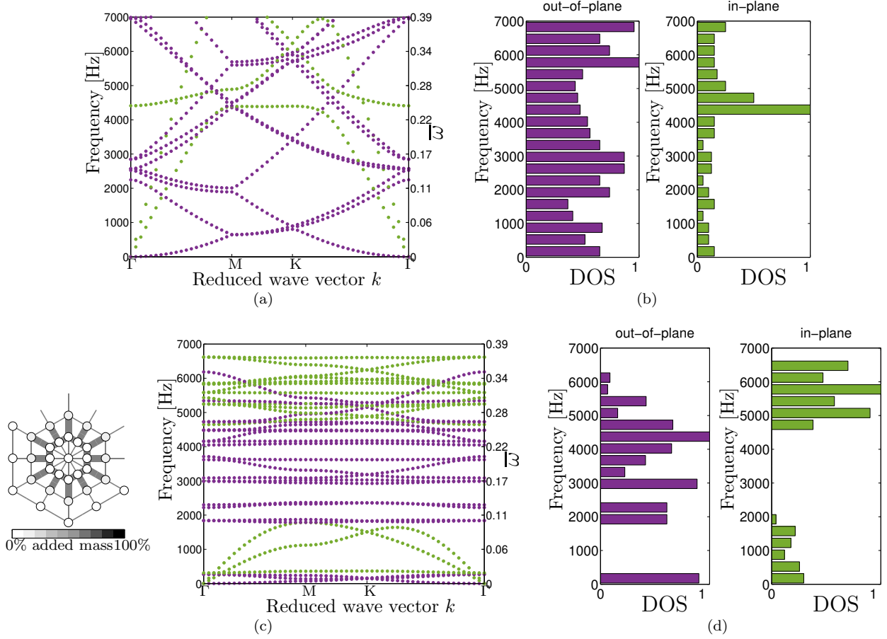
Figure 11: Band diagrams and histograms accounting for (●) out-of-plane and (●) in-plane polarization modes. The initial band diagram (a) and its corresponding propagating frequency histograms (b) show each of the 20 frequency bins with wave modes from each type of polarization. After the optimization, the final band diagram and unit cell (c) – obtained using the optimization objective \varphi^{(p)} (Eq. (10)) – with its corresponding histogram (d) show 13 frequency bins with a single type of polarization and a few with non polarized modes.
