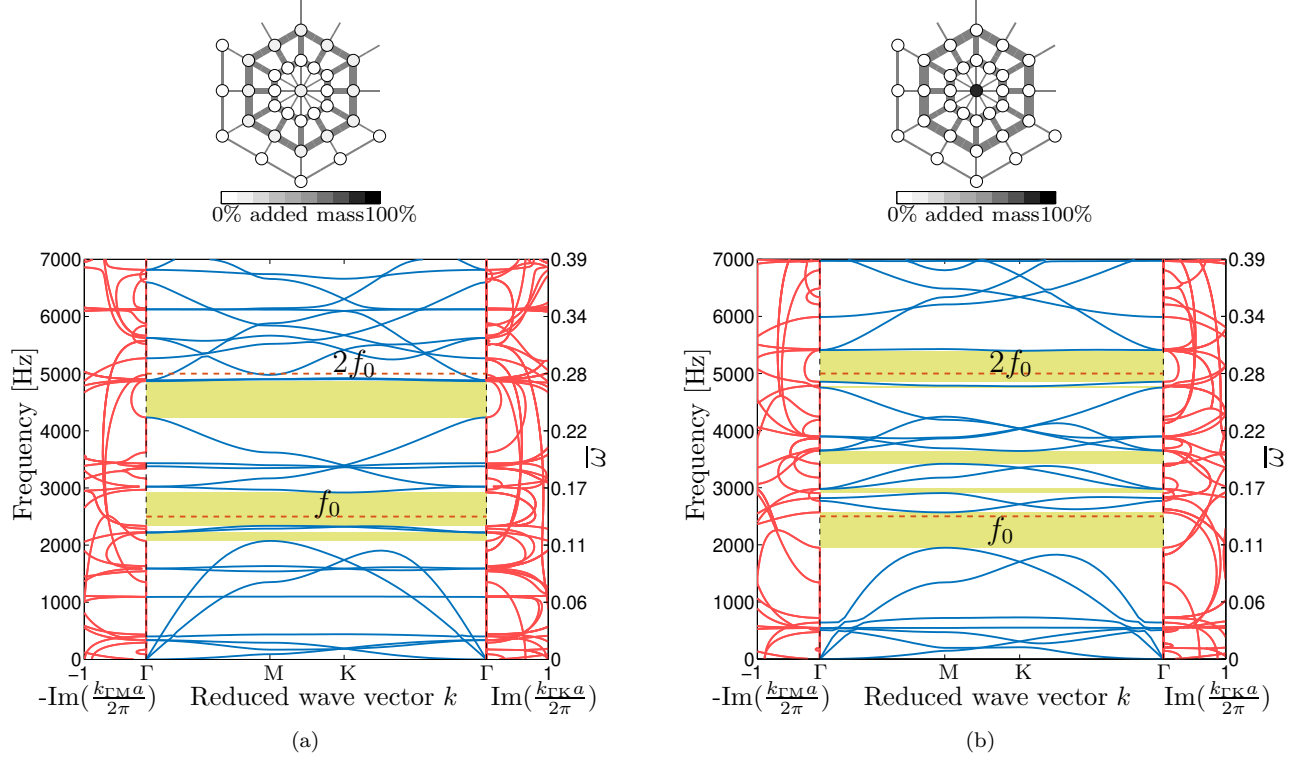
Figure 10: Band diagrams and their corresponding unit cells obtained using the optimization objective that (a) opens a BG only at the fundamental frequency ( \varphi_{\omega_0}^{(\text{fh})} , Eq. (8)) and (b) attenuates all harmonics ( \varphi_{\omega_0}^{(\text{ah})} , Eq. (9)) for f_0 = 2500 Hz. Harmonics are indicated using dashed lines (- -).
