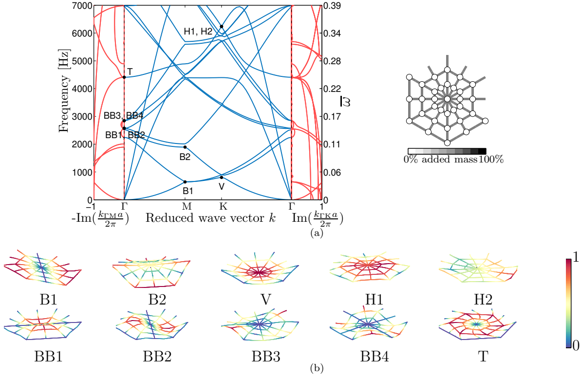
Figure 4: Initial results for the hexagonal lattice structure: (a) band diagram with the real and imaginary parts of the wave vector marked in blue and red, respectively, showing no BGs; (b) mode displacements profiles (colored according to the magnitude of displacement and normalized according to the maximum of displacement in each case): V is an out-of-plane displacement mode, B1 and B2 represent bending modes, BB1 and BB2 represent second-order-like bending modes, BB3 and BB4 represent third-order-like bending modes, H1 and H2 are in-plane displacement modes, and T is a torsional mode.
