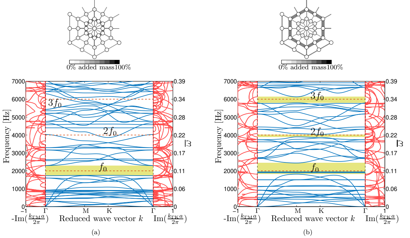
Figure 9: Band diagrams and their corresponding unit cells obtained using the optimization objective that (a) opens a BG only at the fundamental frequency ( \varphi_{\omega_0}^{(\text{fh})} , Eq. (8)) and (b) attenuates all harmonics ( \varphi_{\omega_0}^{(\text{ah})} , Eq. (9)) for f_0 = 2000 Hz. Harmonics are indicated using dashed lines (- -).
