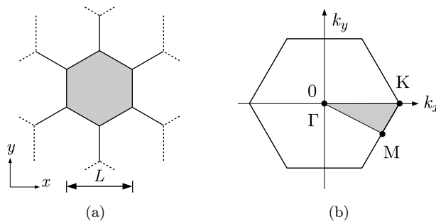
Figure 2: (a) Two-dimensional hexagonal periodic medium with a highlighted unit cell and (b) FBZ with its highlighted IBZ and high symmetry points \Gamma (0,0), M ( \pi/L , -\pi/L\sqrt{3} ), and K ( 4\pi/3L , 0).
